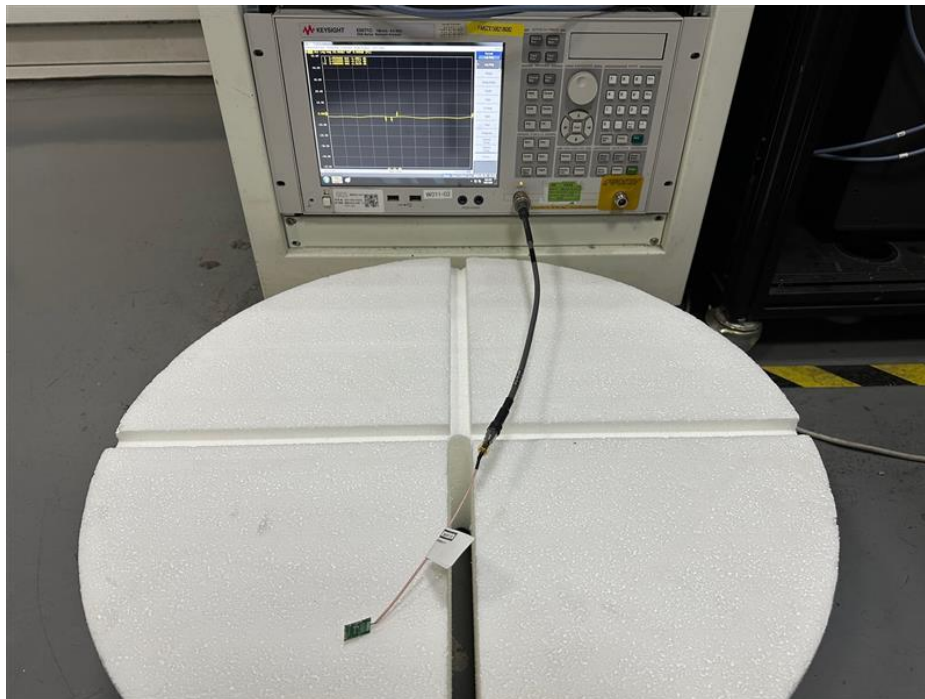
Free Space Impedance Setup #1
