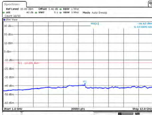
Band71_20MHz_QPSK_133372_1RB#0
