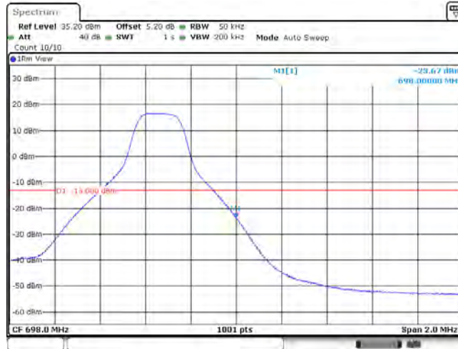
Band71_5MHz_16QAM_133447_25RB#0
