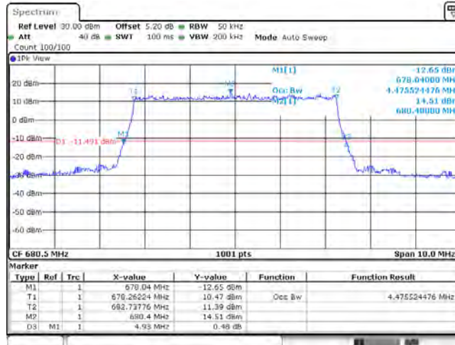
Band71_5MHz_QPSK_133297_25RB#0
