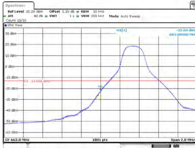
Band71_5MHz_QPSK_133147_1RB#0
