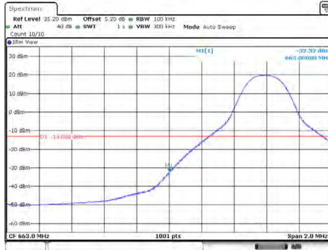
Band71_10MHz_16QAM_133172_50RB#0
