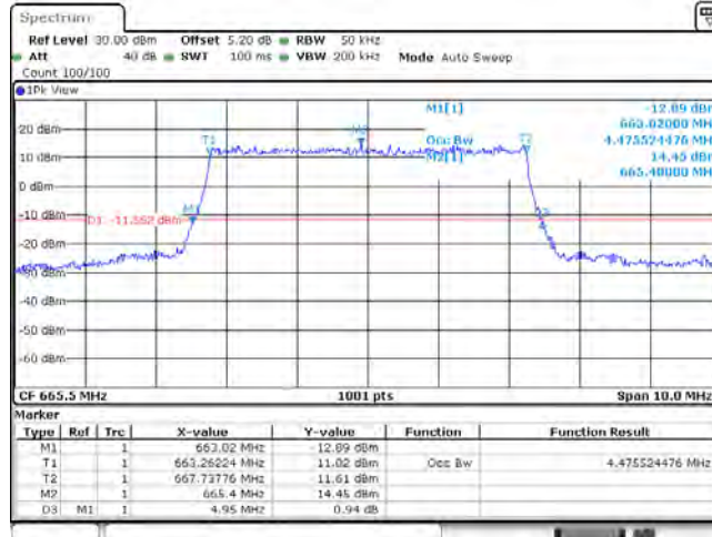
Band71_5MHz_QPSK_133147_25RB#0
