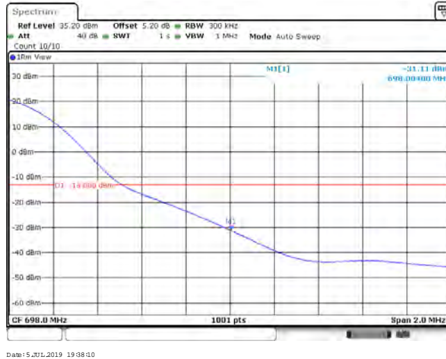
Band71_20MHz_16QAM_133372_100RB#0
