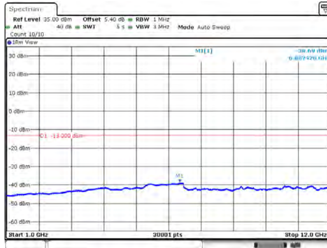
Band71_20MHz_QPSK_133322_1RB#0
