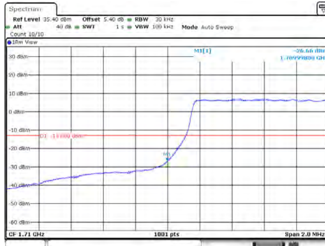
Band66_1.4MHz_16QAM_131979_6RB#0
