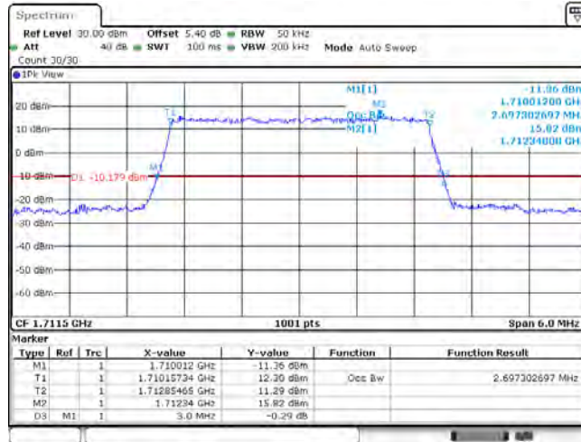
Band66_3MHz_QPSK_132322_15RB#0
