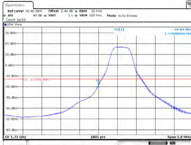
Band66_3MHz_16QAM_131987_15RB#0
