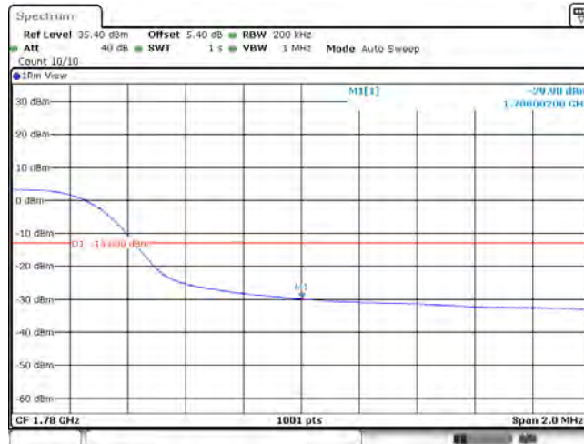
Band66_15MHz_QPSK_132597_75RB#0
