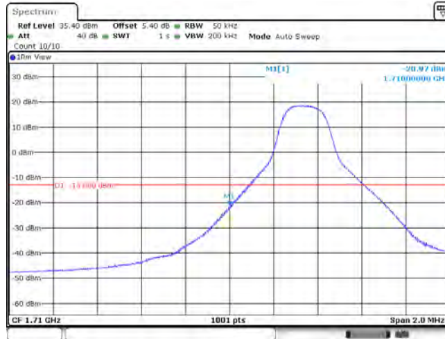
Band66_5MHz_QPSK_131997_25RB#0
