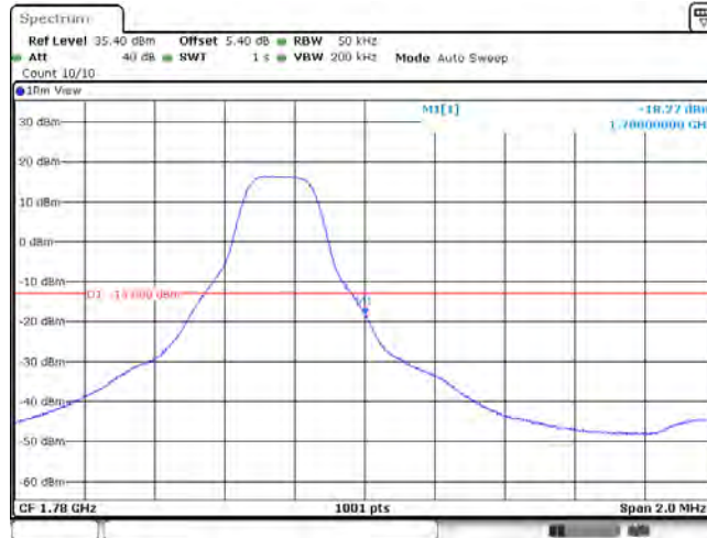
Band66_3MHz_16QAM_132657_15RB#0
