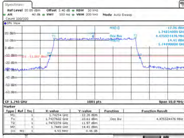
Band66_5MHz_QPSK_132322_25RB#0
