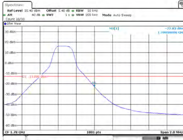
Band66_5MHz_16QAM_132647_25RB#0
