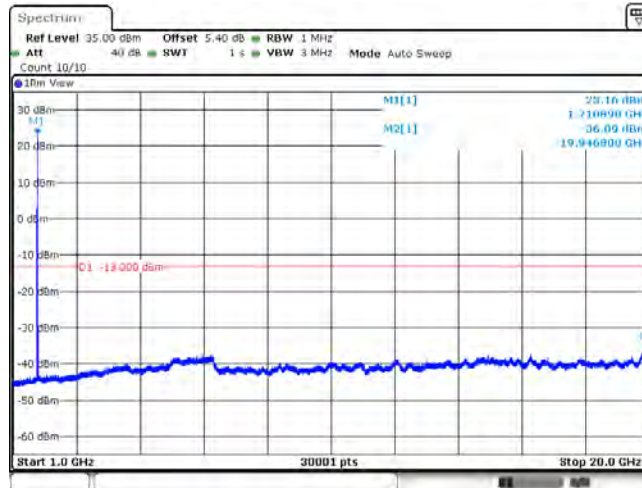
Band66_20MHz_16QAM_132072_1RB#0
