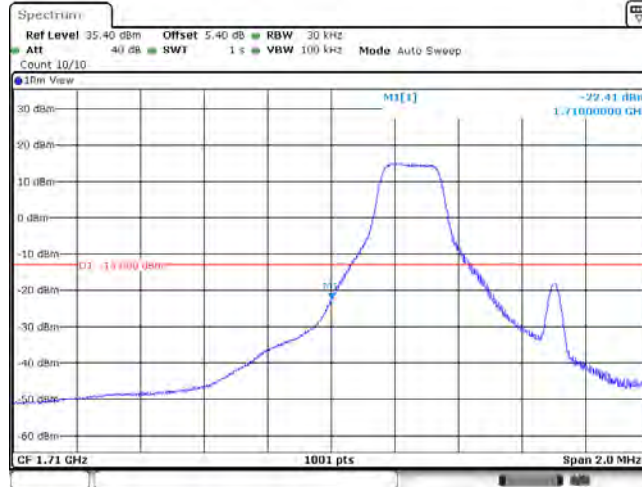
Band66_1.4MHz_16QAM_131979_6RB#0
