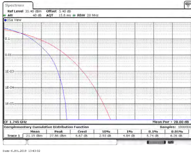
Band66_20MHz_16QAM_132572_100RB#
