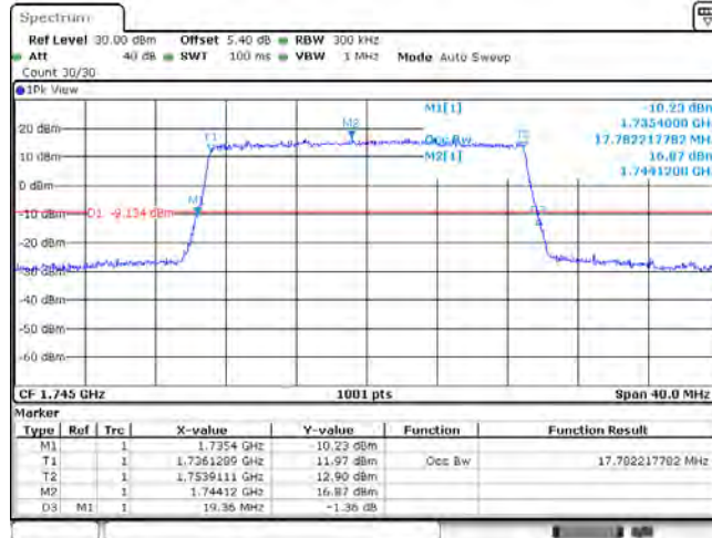
Band66_20MHz_QPSK_132322_100RB#0
