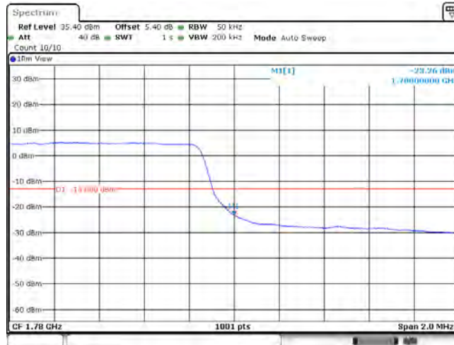
Band66_3MHz_QPSK_132657_15RB#0
