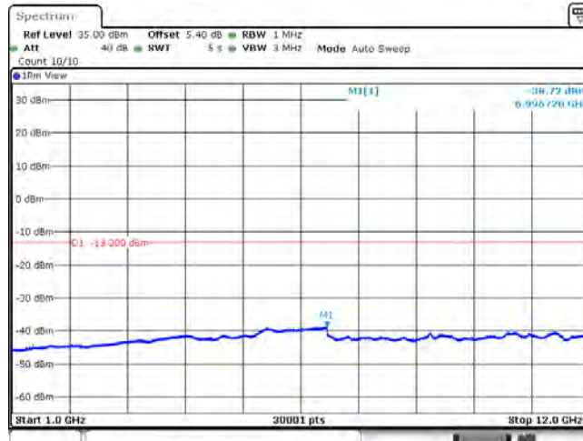
Band12_10MHz_QPSK_23095_1RB#0
