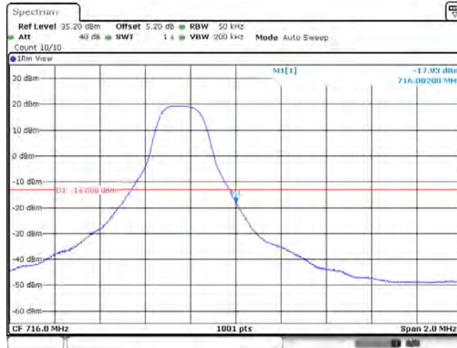
Band12_3MHz_QPSK_23165_15RB#0
