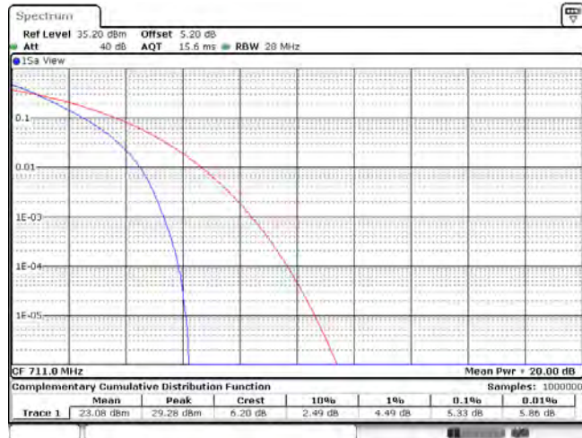
Band12_10MHz_QPSK_23130_50RB#0
