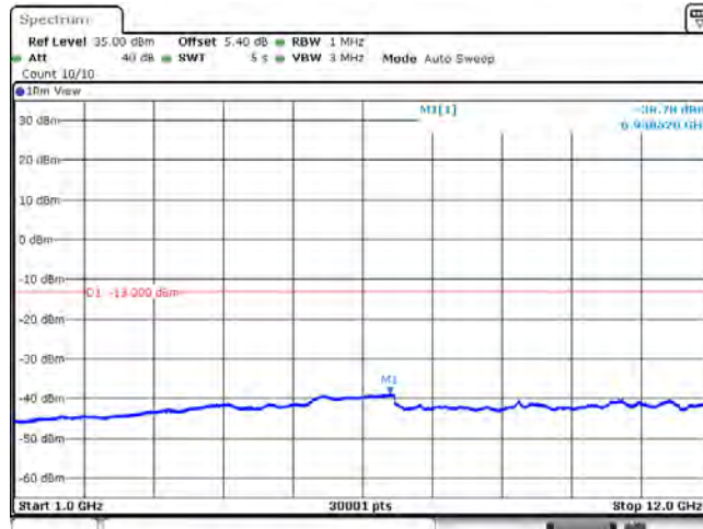
Band12_10MHz_16QAM_23095_1RB#0
