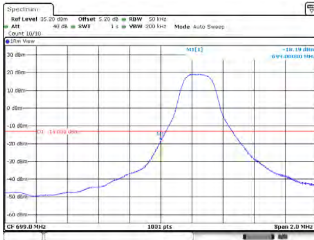
Band12_3MHz_QPSK_23025_15RB#0
