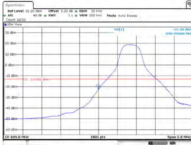
Band12_5MHz_QPSK_23035_25RB#0
