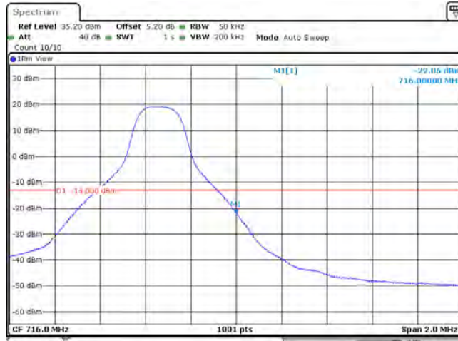
Band12_5MHz_QPSK_23155_25RB#0
