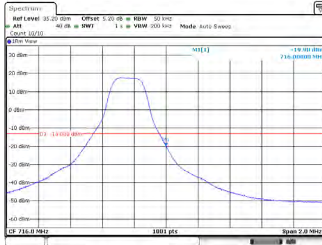
Band12_3MHz_16QAM_23165_15RB#0
