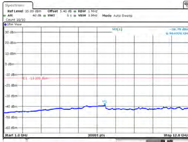
Band12_10MHz_16QAM_23060_1RB#0
