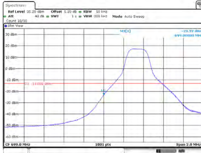
Band12_5MHz_16QAM_23035_25RB#0
