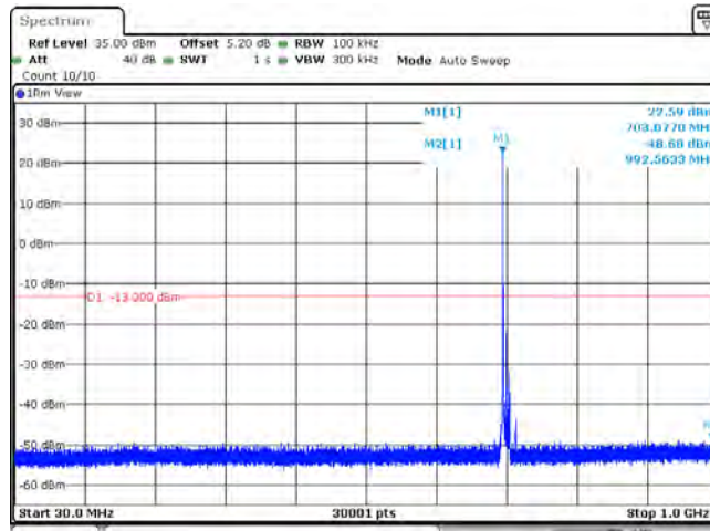
Band12_10MHz_16QAM_23095_1RB#0
