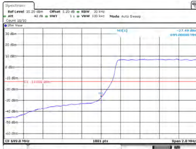
Band12_1.4MHz_16QAM_23017_6RB#0
