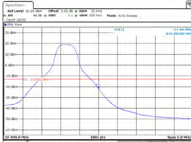
Band5_5MHz_QPSK_20625_25RB#0
