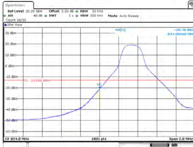
Band5_5MHz_QPSK_20425_25RB#0
