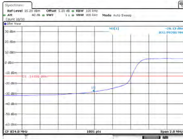
Band5_10MHz_QPSK_20450_50RB#0
