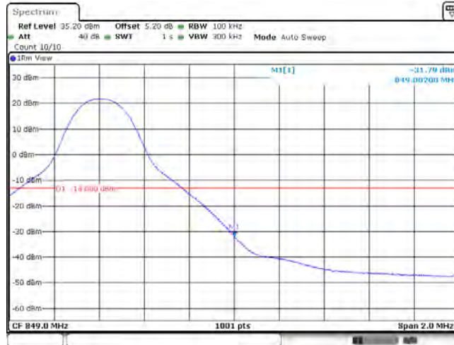
Band5_10MHz_QPSK_20600_50RB#0
