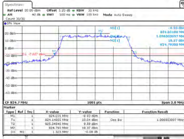
Band5_1.4MHz_QPSK_20407_6RB#0
