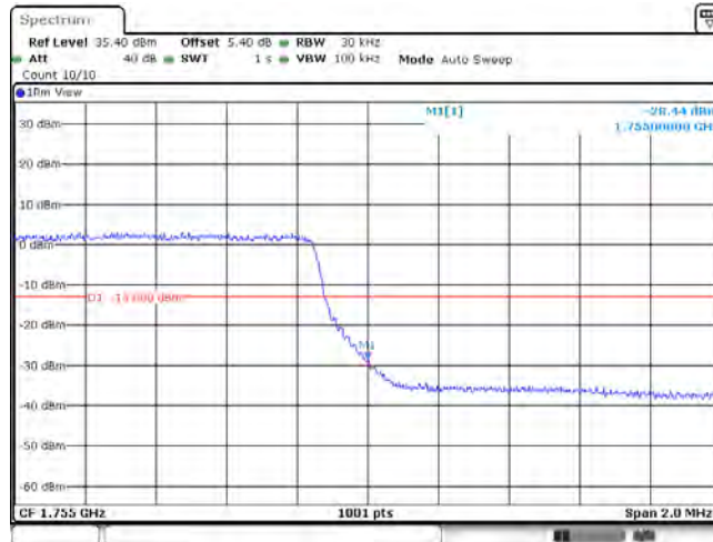
Band4_3MHz_16QAM_20385_15RB#0
