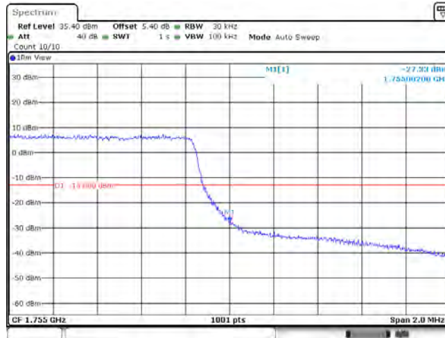
Band4_1.4MHz_16QAM_20393_6RB#0
