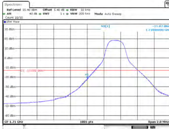
Band4_5MHz_QPSK_19975_25RB#0
