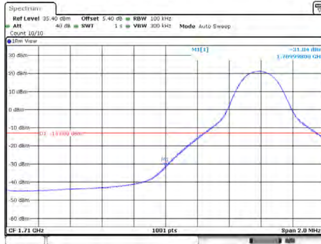
Band4_10MHz_QPSK_20000_50RB#0
