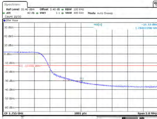
Band4_10MHz_QPSK_20350_50RB#0
