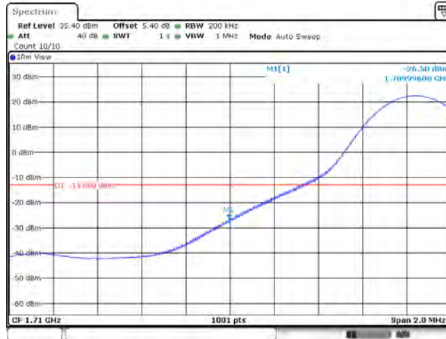
Band4_15MHz_QPSK_20025_75RB#0
