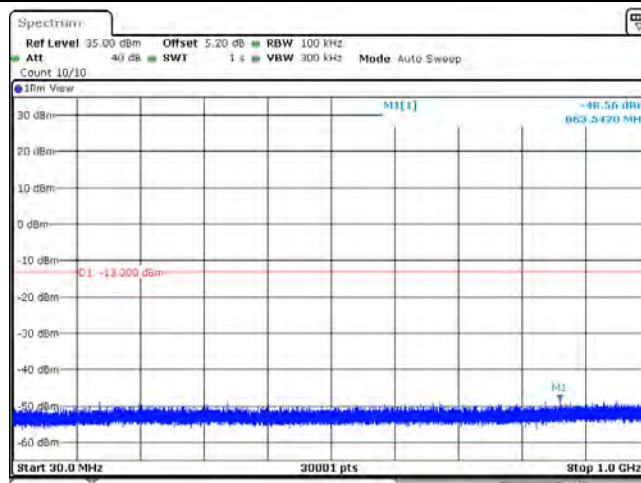
Band4_20MHz_QPSK_20050_1RB#0
