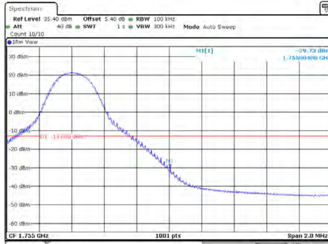
Band4_10MHz_QPSK_20350_50RB#0
