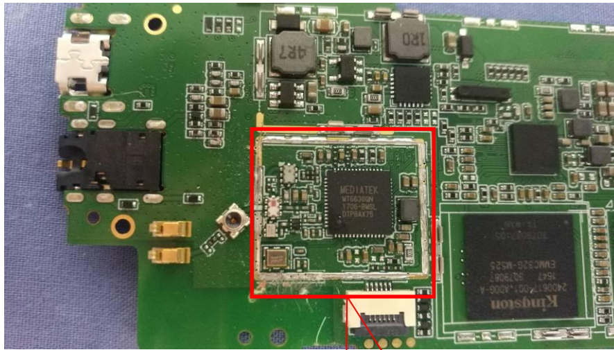
GPS&BT&2.4G & 5G WIFI RF Module
