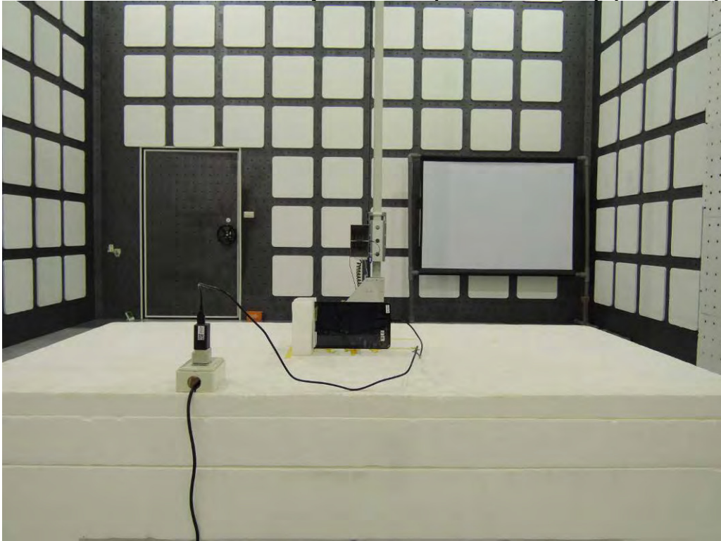
Radiated Emission Set up Photos (Above 1GHz) (E1 Plan)
