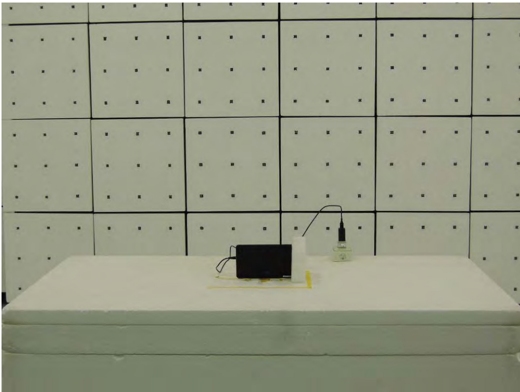
Radiated Emission Set up Photos (Below 1GHz)(E2 Plan)
