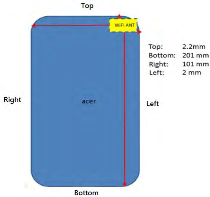
Fig.9 Antenna position of EUT (Back view)
