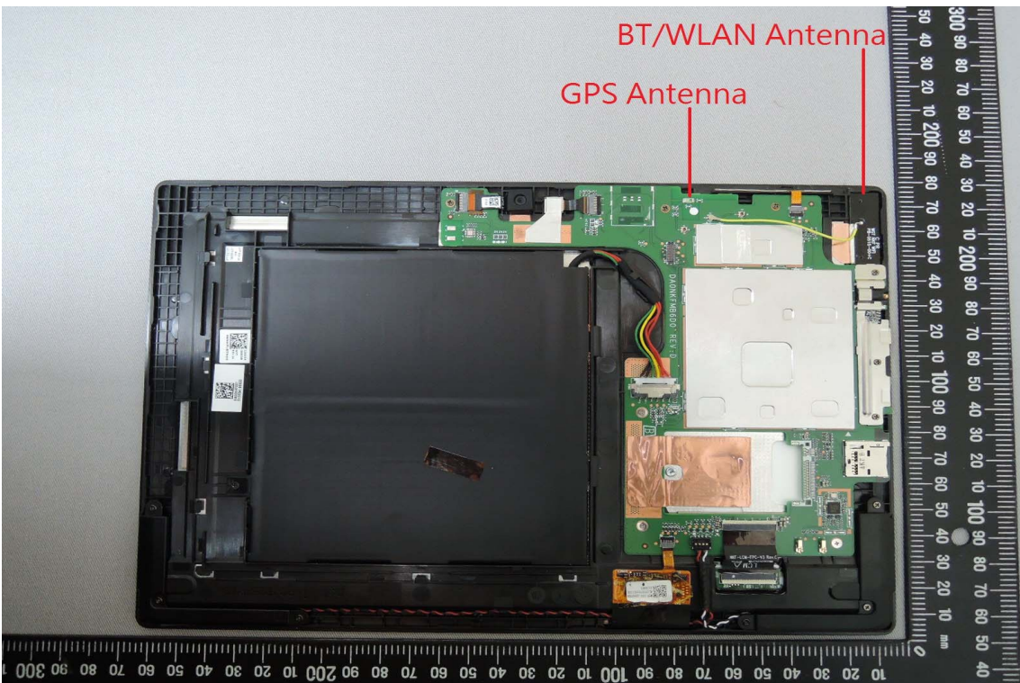
GPS & BT & WLAN Antenna Location
