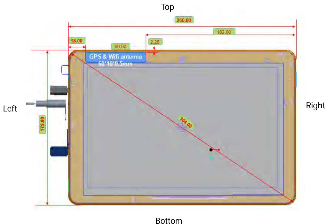
Fig.8 Antenna position of EUT
