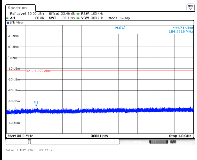
CSE Plot on Ch 00 between 30MHz ~ 1 GHz
