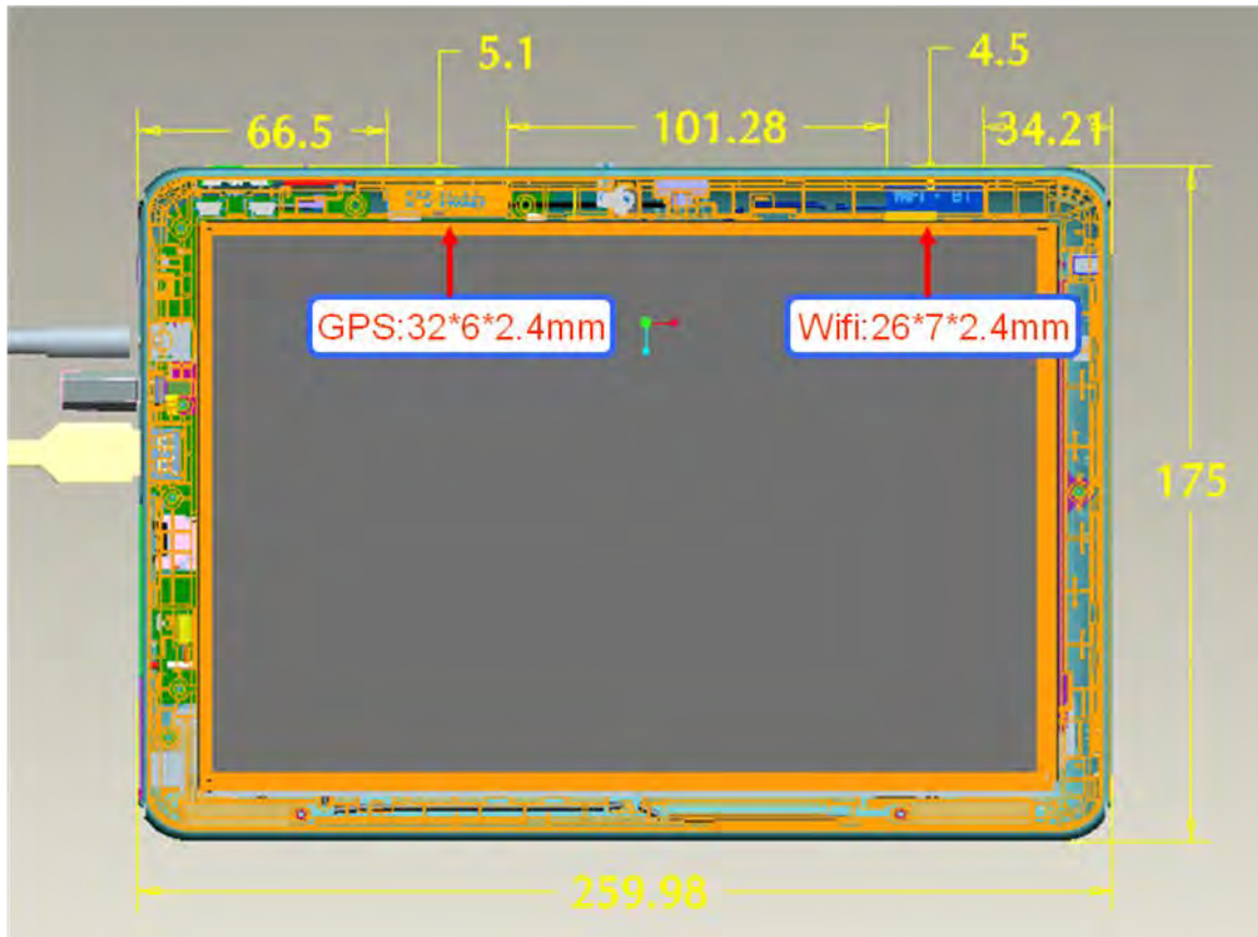
Fig.8 Antenna position of EUT
