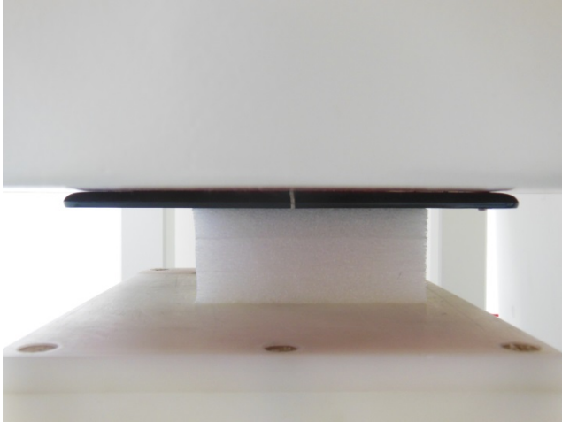
Bottom Face, Test Separation 0 cm for Sample 2
