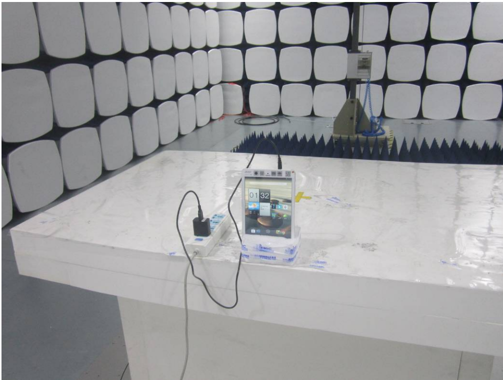
Radiated Spurious Emissions Test Setup Above 1GHz -Front View(Adapter1)
