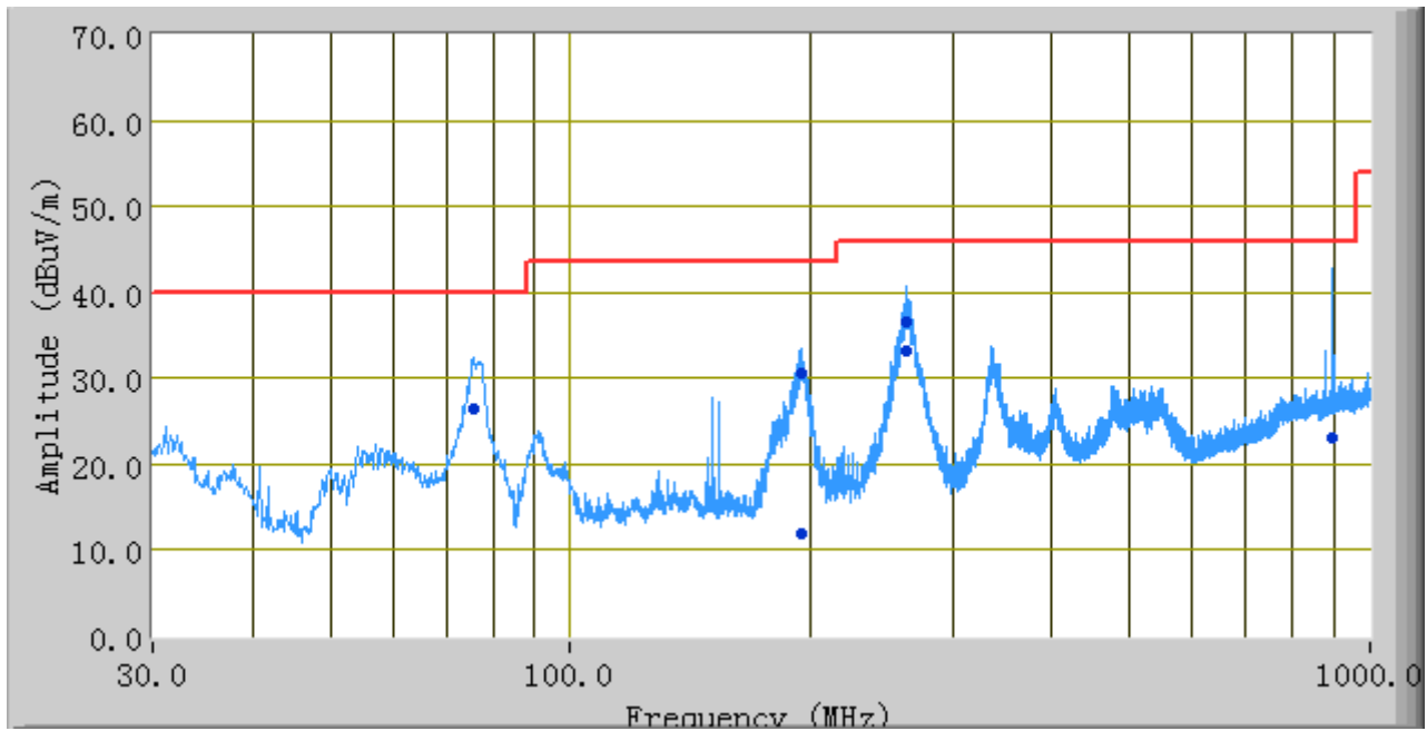
Vertical & Horizontal Polarity Plot @3m
