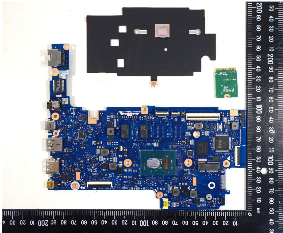
Internal View of EUT – 5
