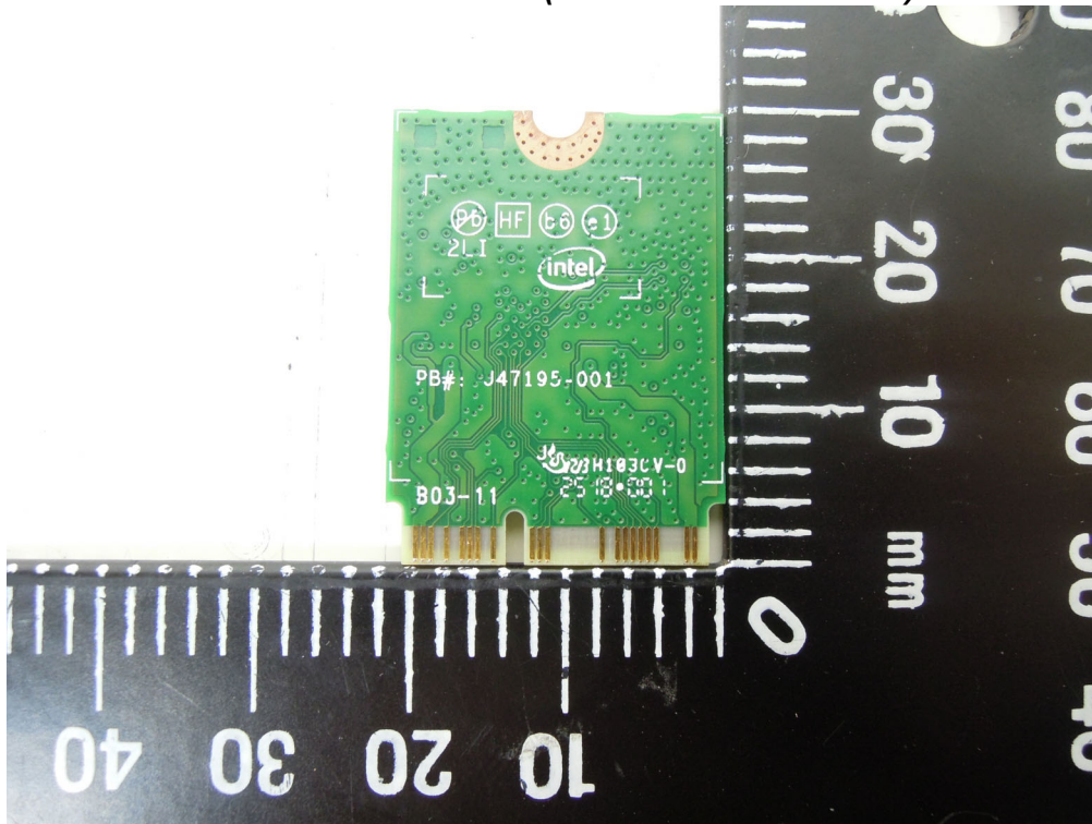
WLAN / BT Module-3 (Model No.: 9560NGW)
