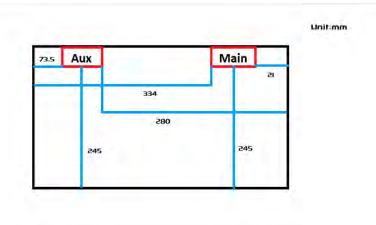
Fig.8 Antenna position of EUT
