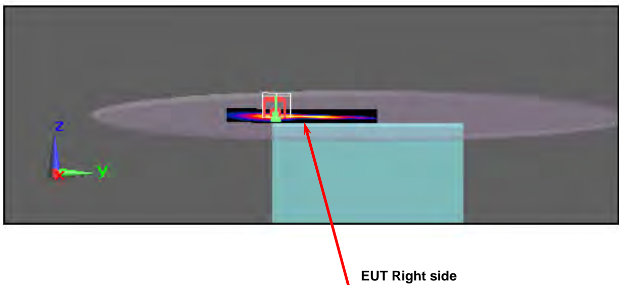
Figure 3. Body SAR Test Setup (Flat Section)_ Tablet Mode LCD Right side Close Body
