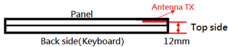
Fig.13 Antenna location of EUT (laptop mode)
