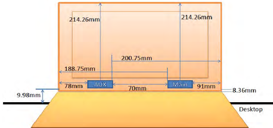
Fig.6 Antenna position of EUT
