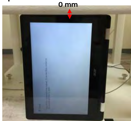
Fig.7 EUT Right side to flat phantom
