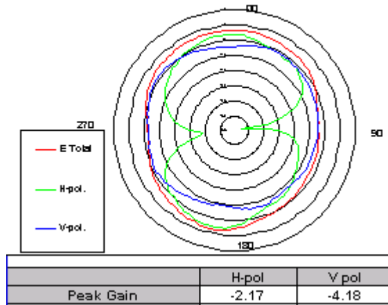
WWAN MAIN antenna @900 MHz
