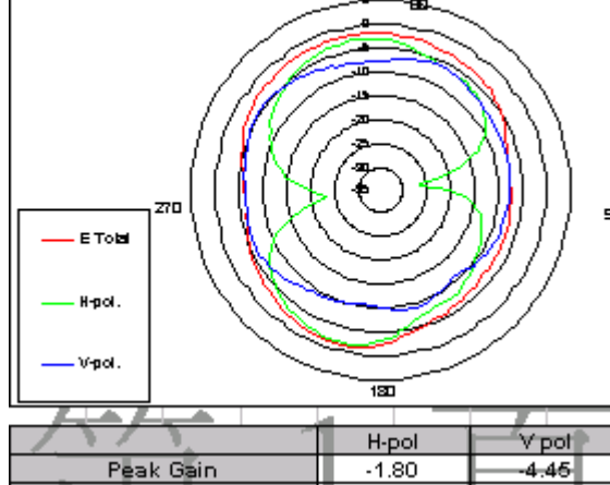
WWAN MAIN antenna @915 MHz
