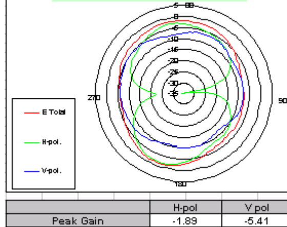
WWAN MAIN antenna @925 MHz
