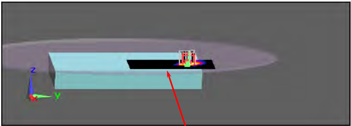
Figure 2. Body SAR Test Setup (Flat Section) _Tablet Mode Bottom Close Body
