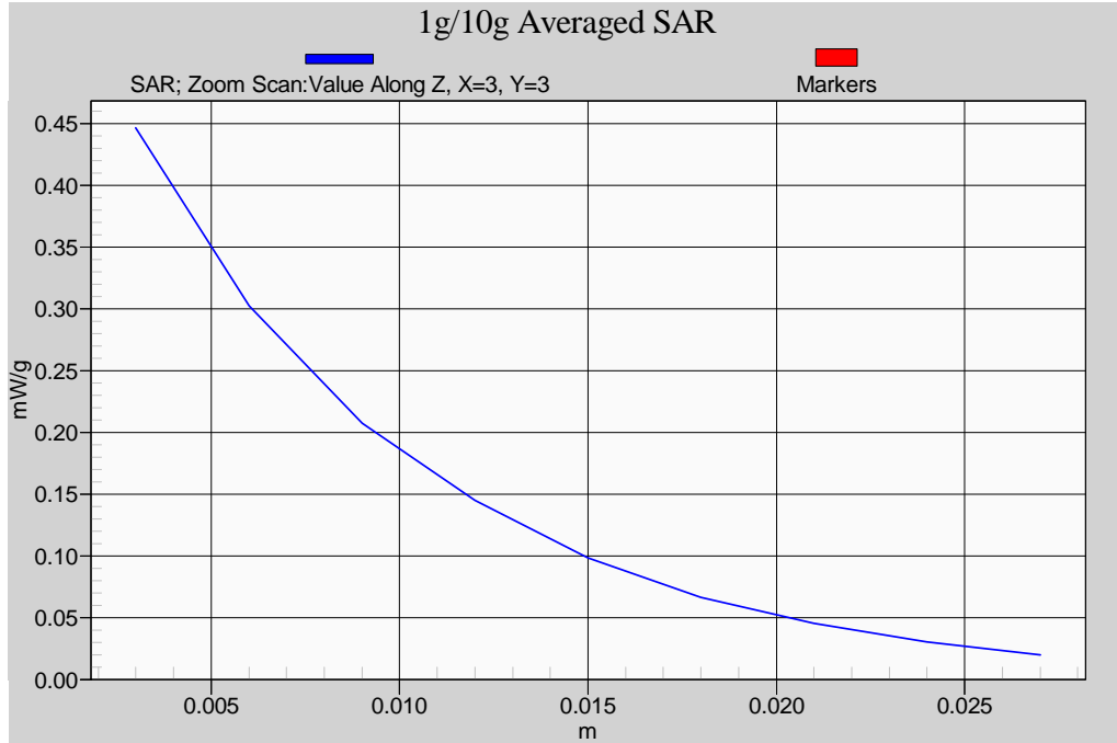
Z-axis Plot of Flat WLAN 802.11g CH 6 (Rate 6M)
