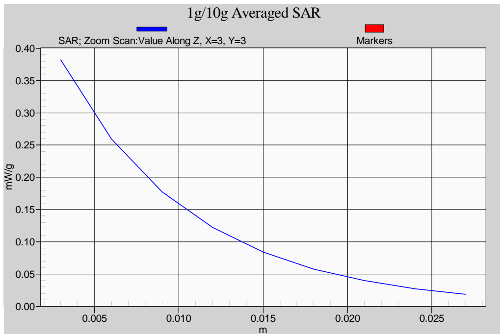
Z-axis Plot of Flat WLAN 802.11n CH 6 (Rate 6.5M)
