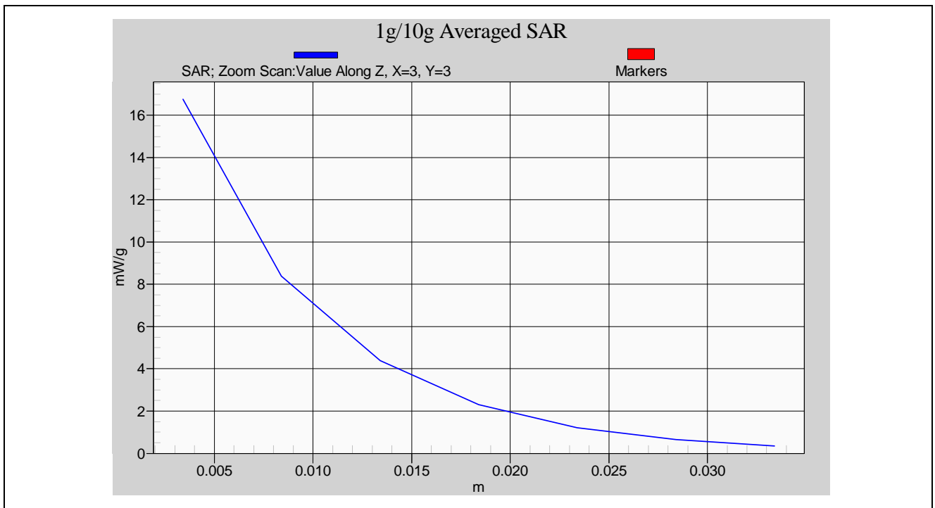
Body-Tissue-Simulating-Liquid 2450MHz_ 11/05/2009
