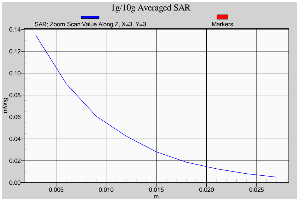
Z-axis Plot of Flat WLAN 802.11n CH 6 (Rate 13.5M)
