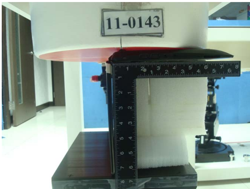
Figure 2. Body SAR Test Setup (Bottom Close Body)_Chain1
