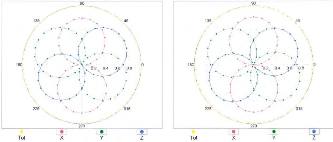
f=600 MHz,TEM
