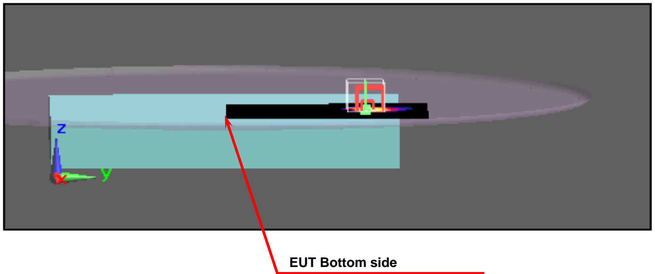
Figure 2. Body SAR Test Setup (Flat Section) _Tablet Mode Bottom Close Body
