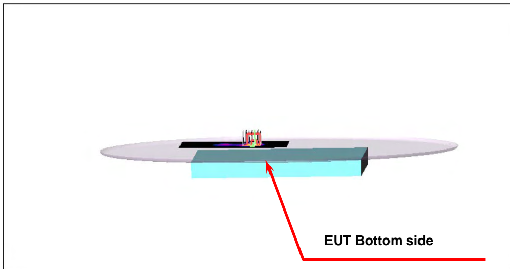
Figure 1. Body SAR Test Setup (Flat Section) Host: LCD Open 90° Bottom Close Body
