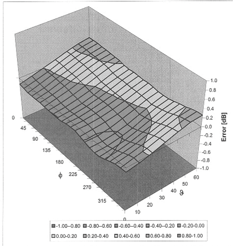
Uncertainty of Spherical Isotropy Assessment: \pm 2.6\% ( k=2 )
