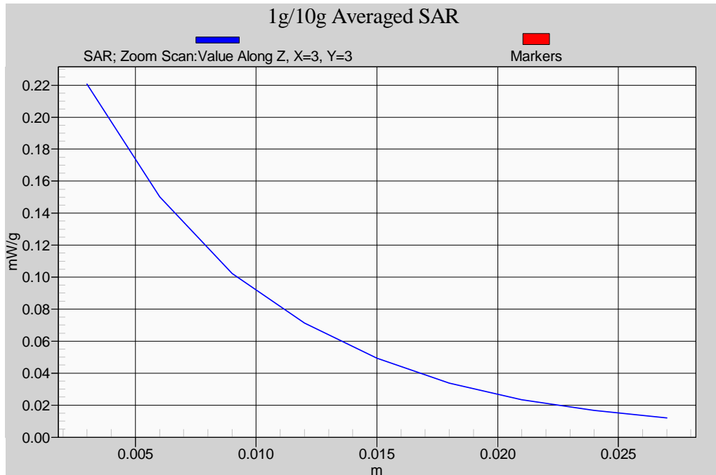
Z-axis Plot of Flat WLAN 802.11b CH 01 (Rate 1M) _ LCD Tip Close Body
