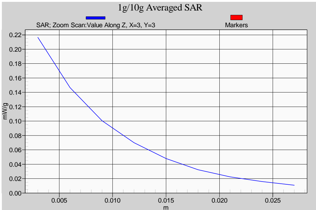
Z-axis Plot of Flat WLAN 802.11g CH 06 (Rate 6M) _ LCD Tip Close Body
