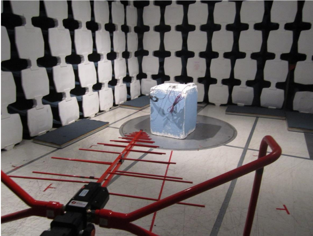
Radiated Emission - 30-1000MHz
