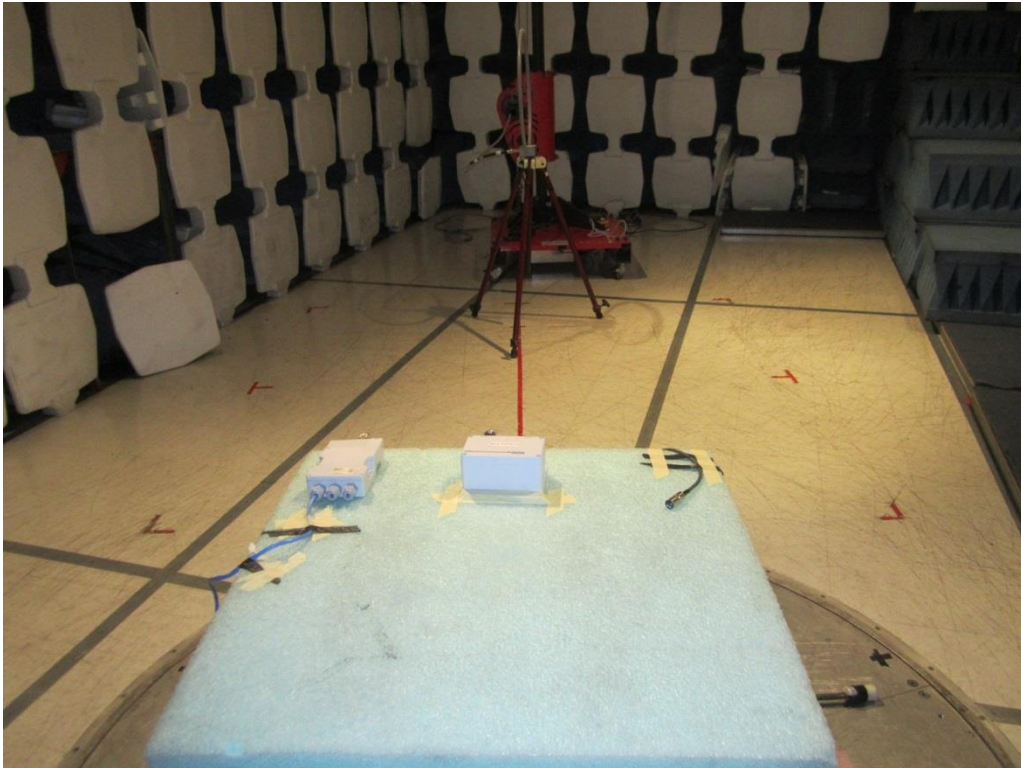
Radiated Emission - 0.15-5MHz
