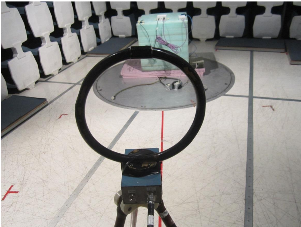
Radiated Emission - 5-30MHz
