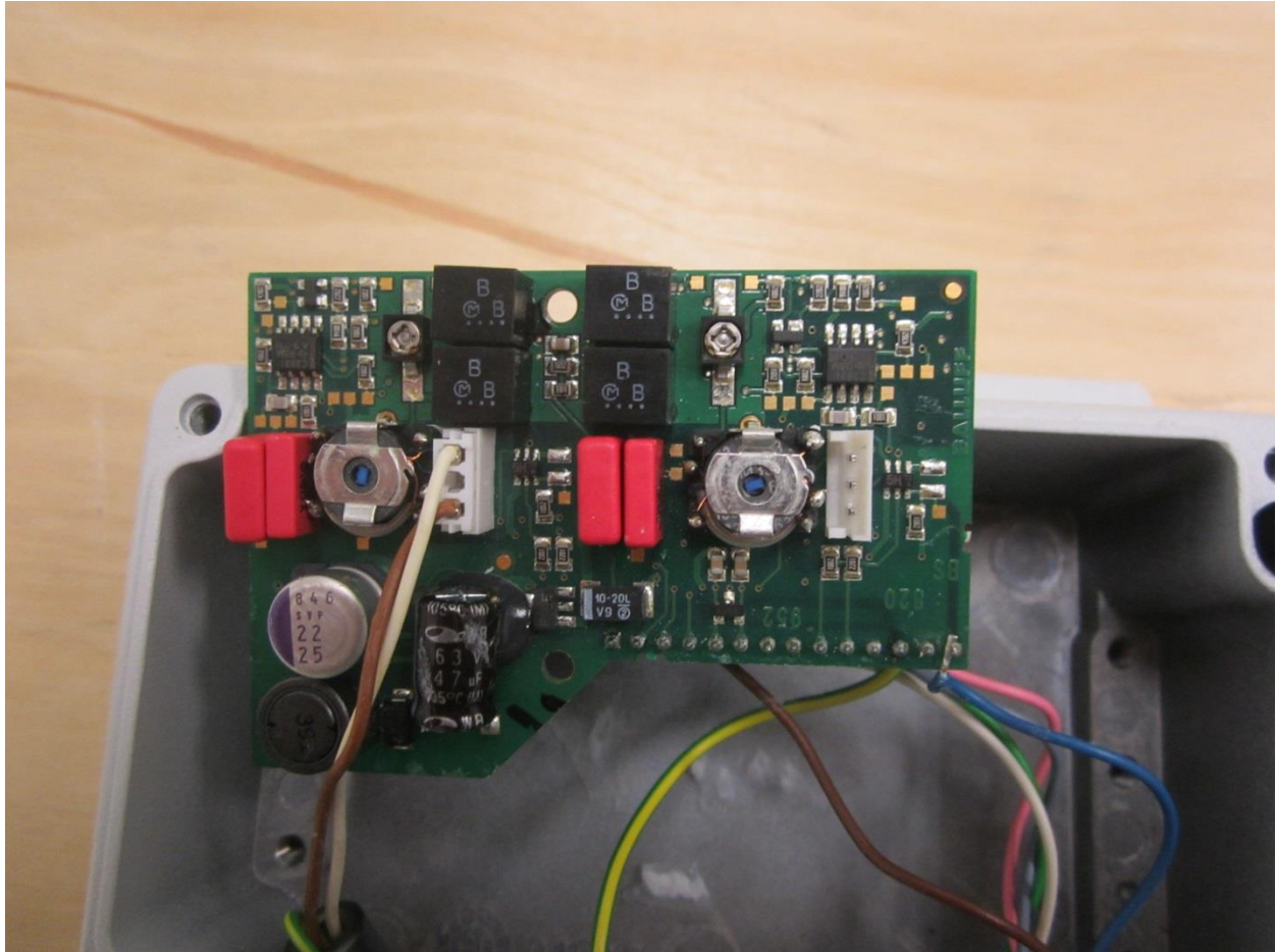
Component side of the module inside the host used during testing – View 2
