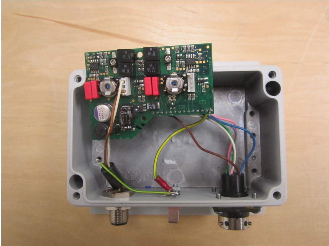
Component side of the module inside the host used during testing – View 1
