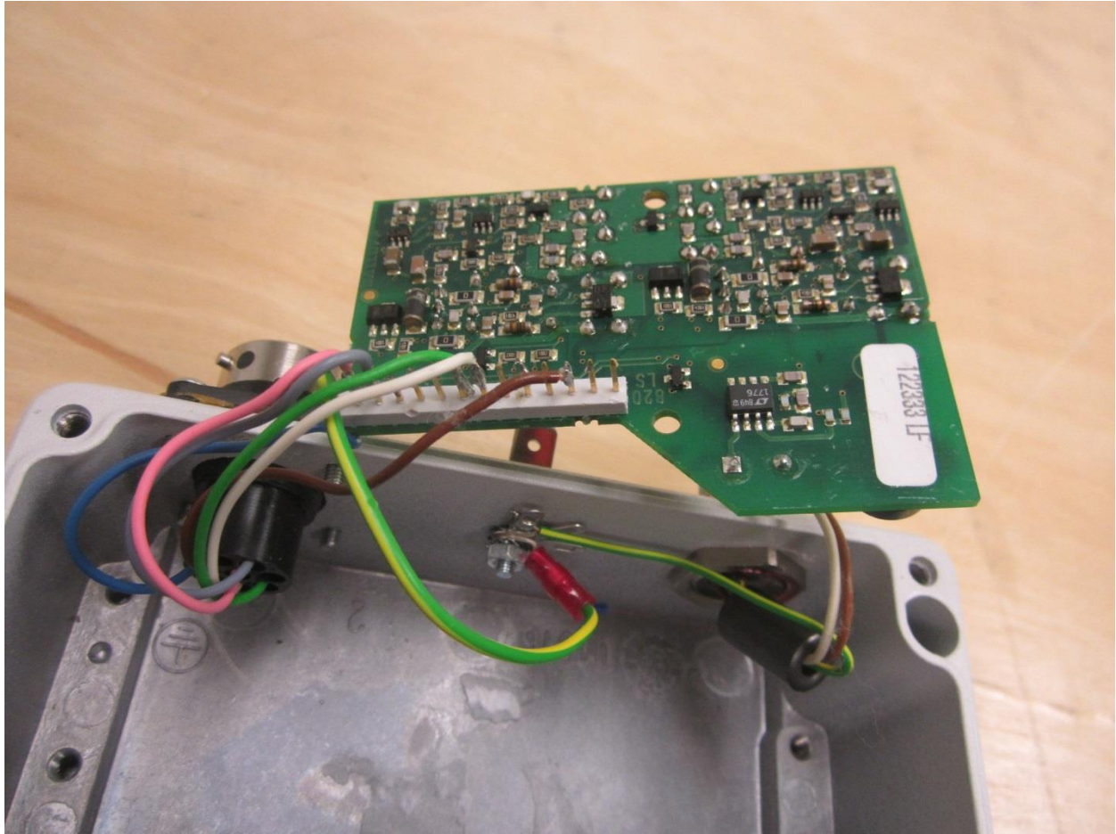
PCB side of the module inside the host used during testing – View 2
