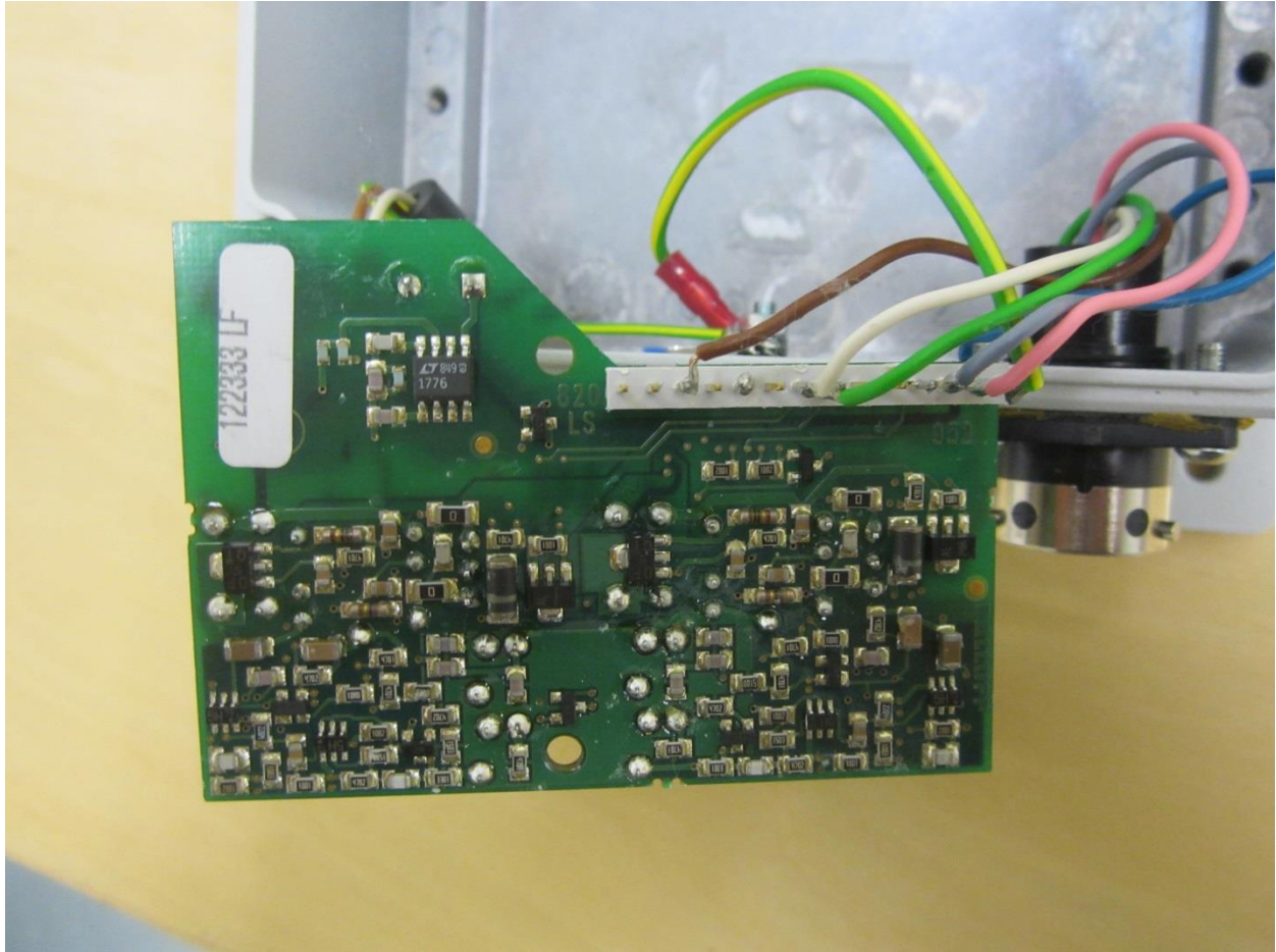
PCB side of the module inside the host used during testing – View 1
