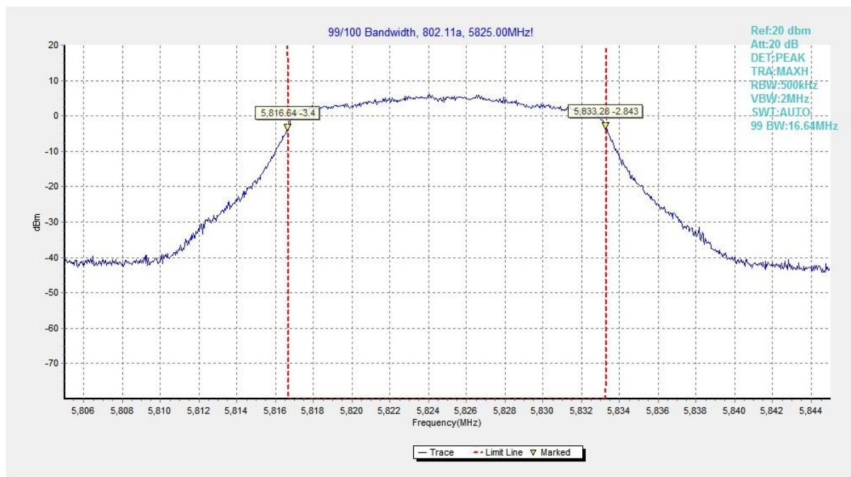
Fig. 38 99% Occupied Bandwidth (802.11a, 5825MHz)
