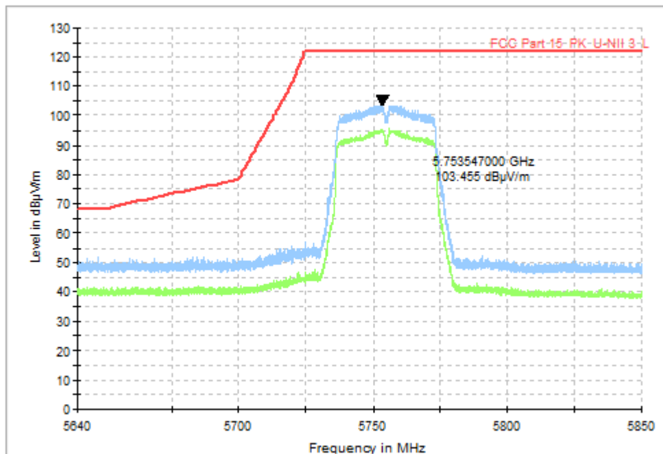
Fig. 63 Band Edges (802.11n-HT40, CH151 5755MHz)
