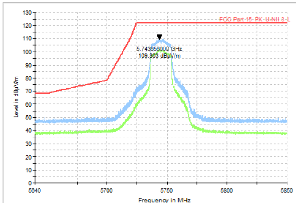
Fig. 57 Band Edges (802.11a, CH149 5745MHz)
