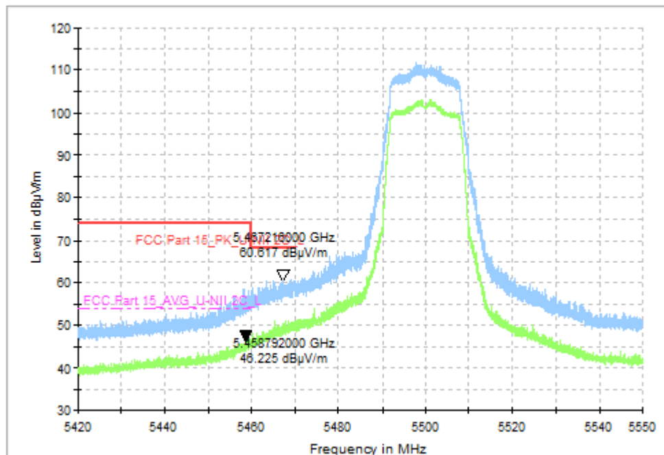
Fig. 55 Band Edges (802.11a, CH100 5500MHz)
