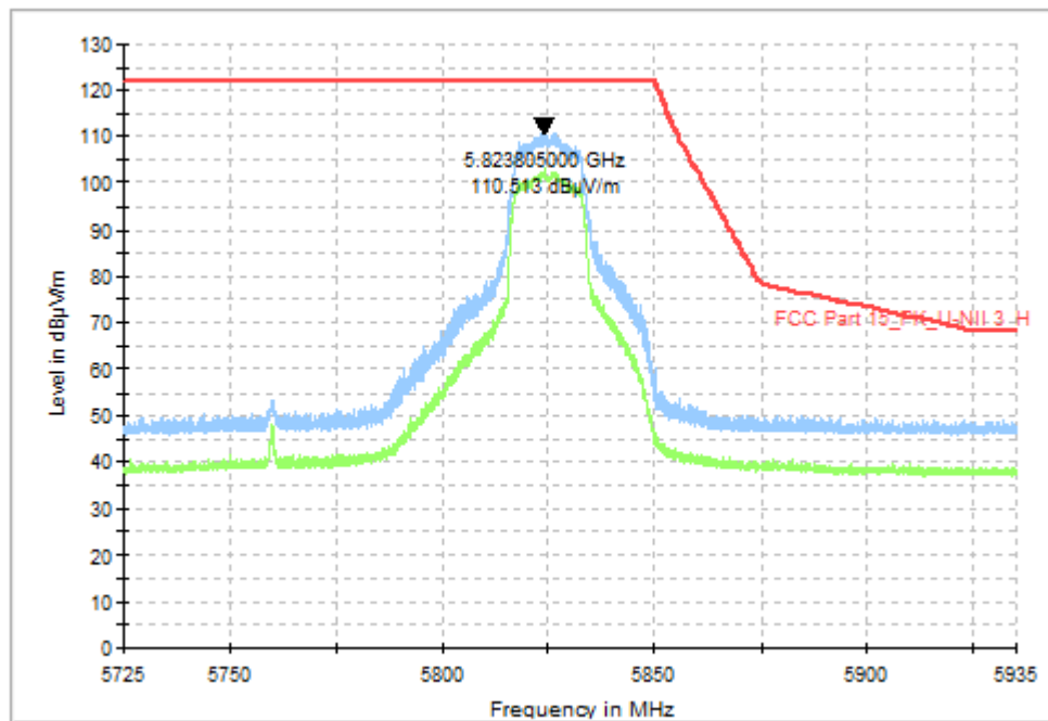
Fig. 58 Band Edges (802.11a, CH165 5825MHz)
