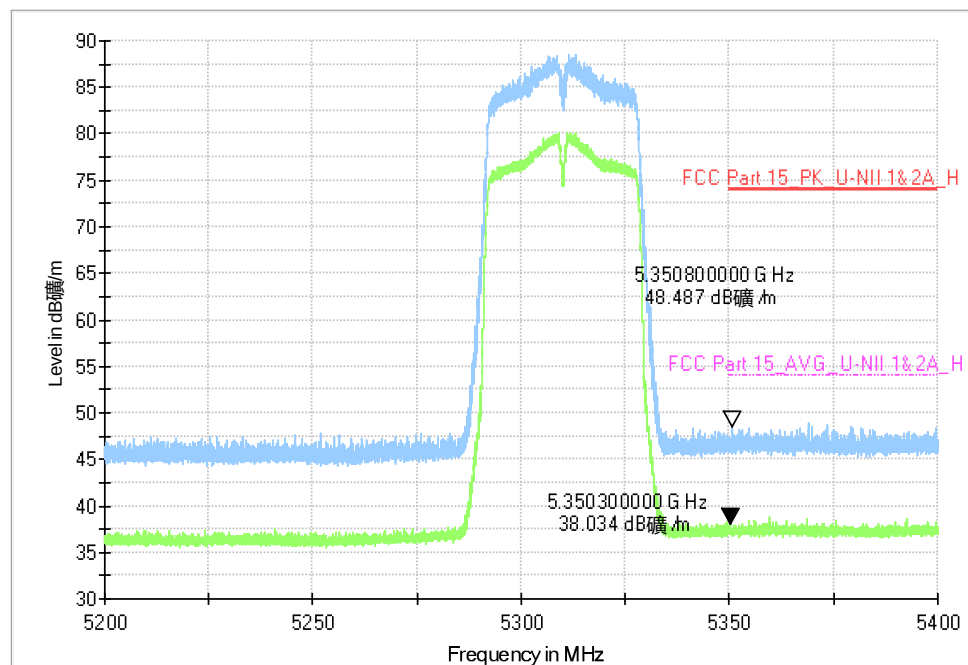
Fig. 60 Band Edges (802.11n-HT40, CH62 5310MHz)
