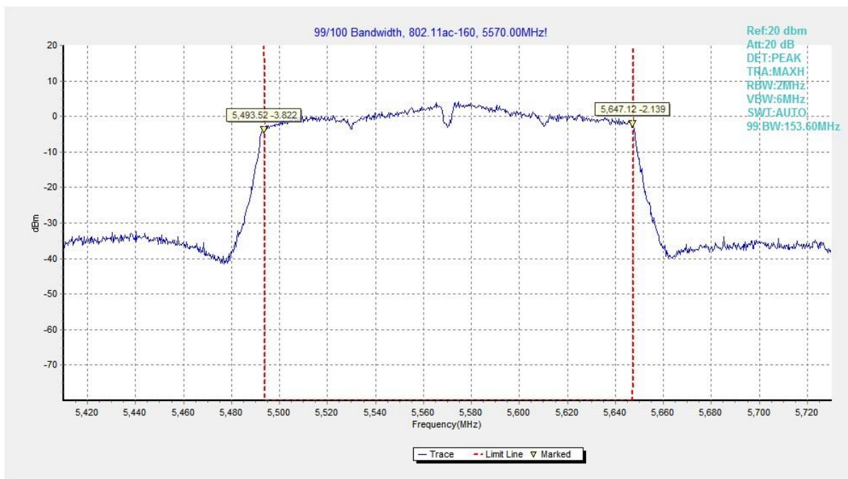
Fig. 52 99% Occupied Bandwidth (802. 11ac-VHT160, 5570MHz)
