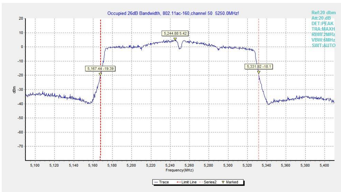
Fig. 19 Occupied 26dB Bandwidth (802. 11ac-VHT160, 5250MHz)
