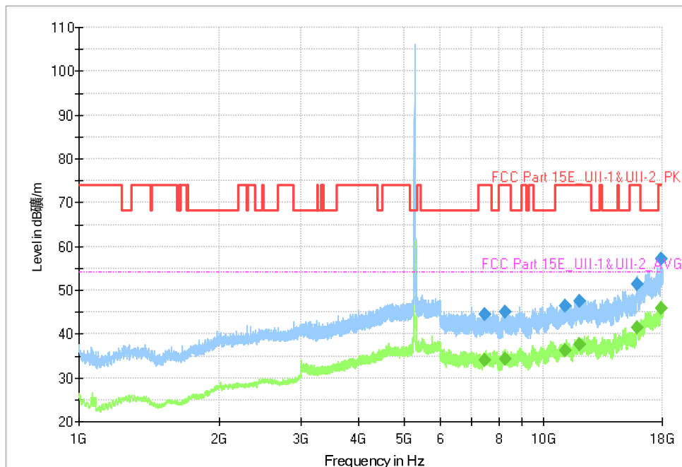
Fig. 75 Transmitter Spurious Emission (802.11a, CH56 5280MHz)
