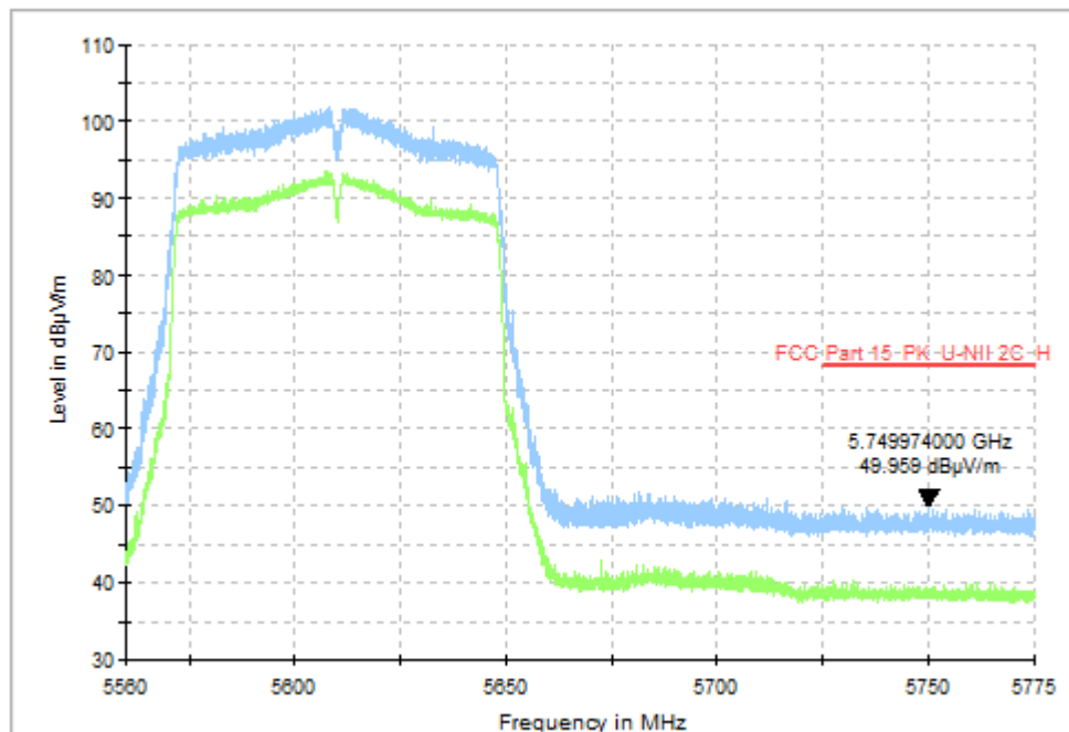
Fig. 67 Band Edges (802.11ac-VHT80, CH122 5610MHz)
