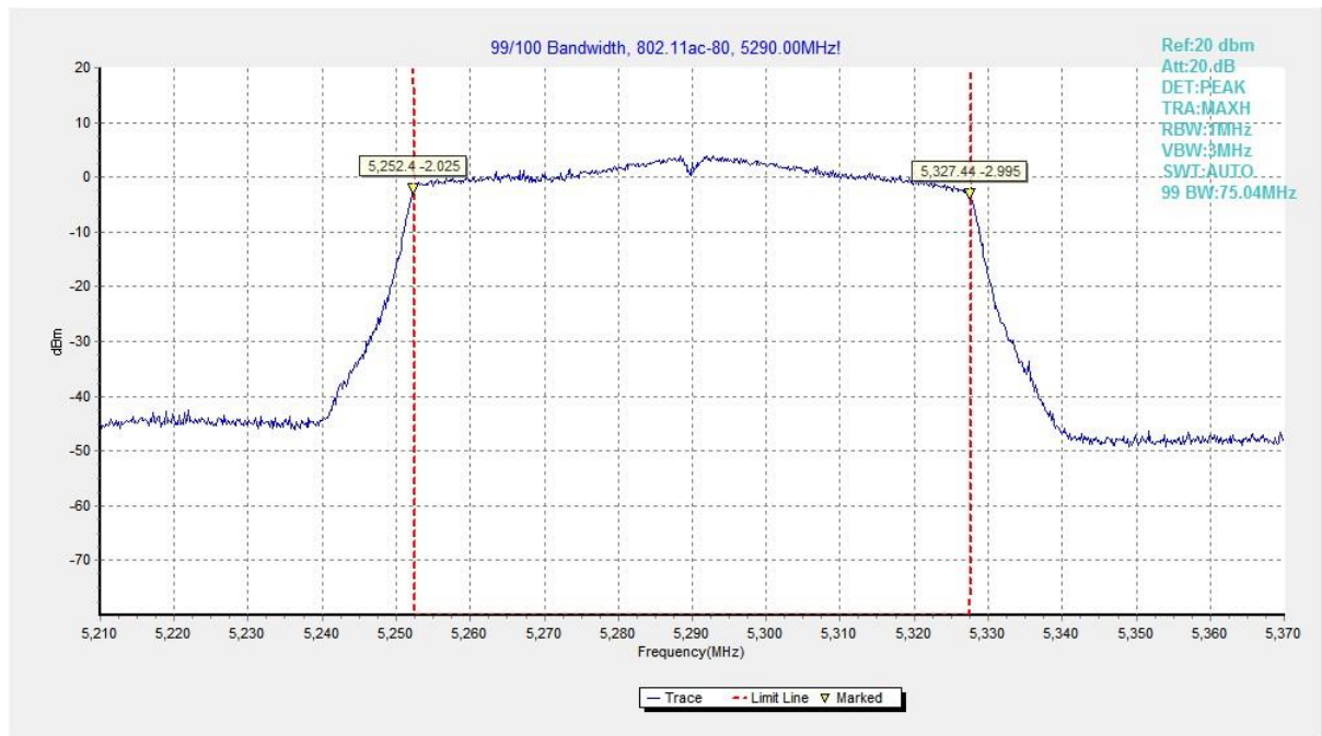
Fig. 48 99% Occupied Bandwidth (802. 11ac-VHT80, 5290MHz)
