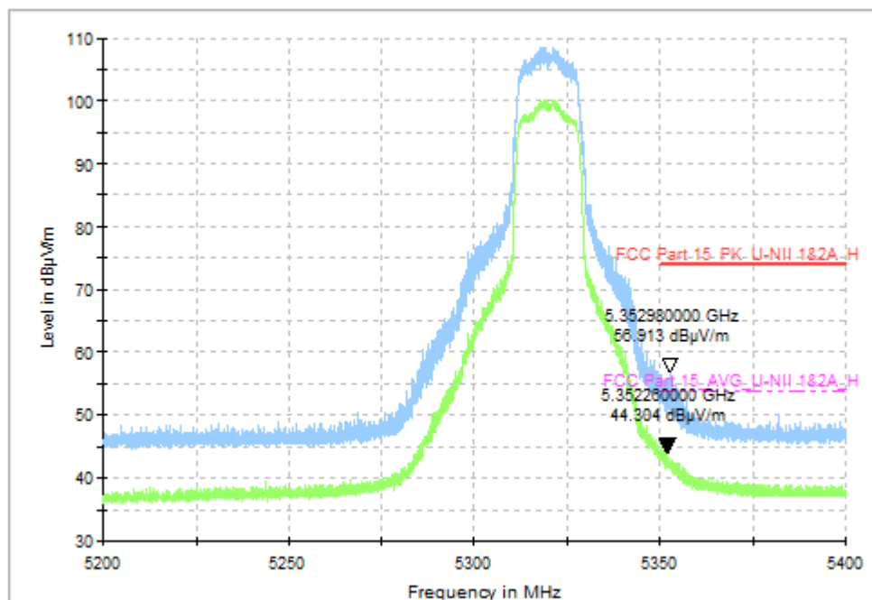
Fig. 54 Band Edges (802.11a, CH64 5320MHz)
