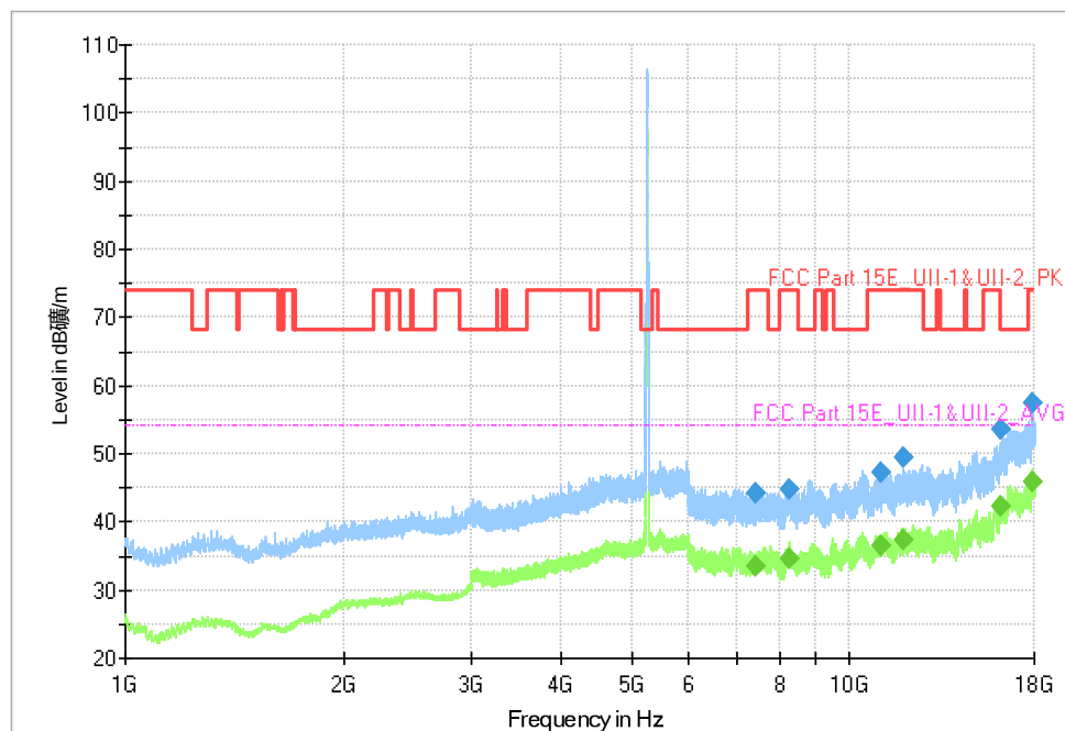
Fig. 74 Transmitter Spurious Emission (802.11a, CH52 5260MHz)
