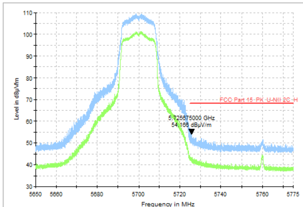
Fig. 56 Band Edges (802.11a, CH140 5700MHz)
