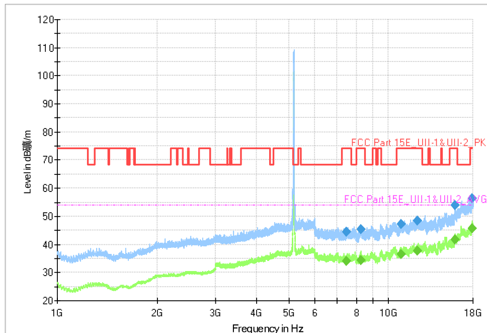
Fig. 71 Transmitter Spurious Emission (802.11a, CH36 5180MHz)
