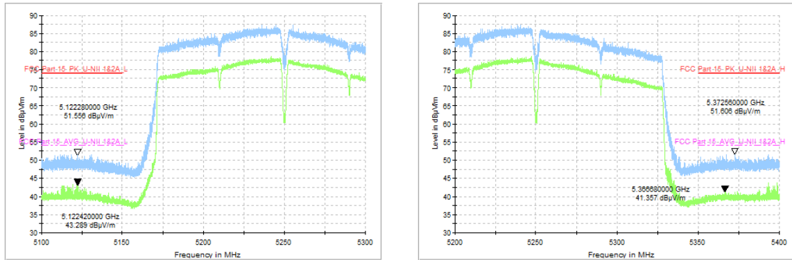
Fig. 69 Band Edges (802.11ac-VHT160, CH50 5250MHz)
