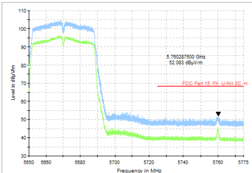
Fig. 62 Band Edges (802.11n-HT40, CH134 5670MHz)
