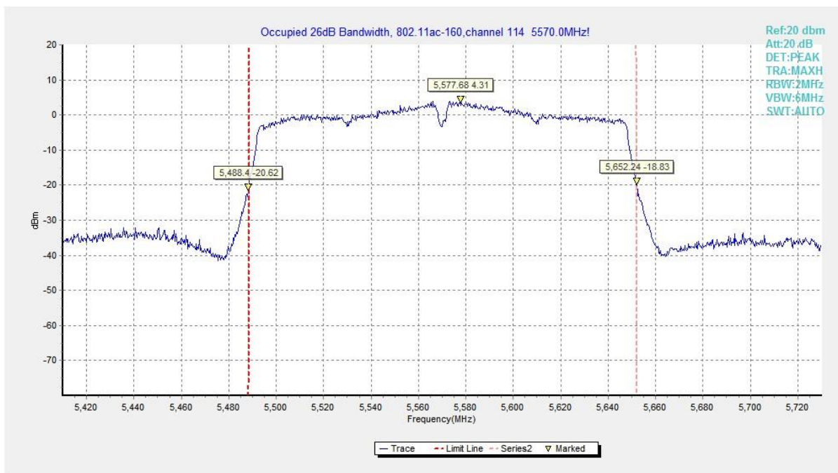
Fig. 20 Occupied 26dB Bandwidth (802. 11ac-VHT160, 5570MHz)
