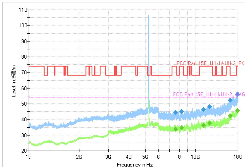
Fig. 73 Transmitter Spurious Emission (802.11a, CH48 5240MHz)
