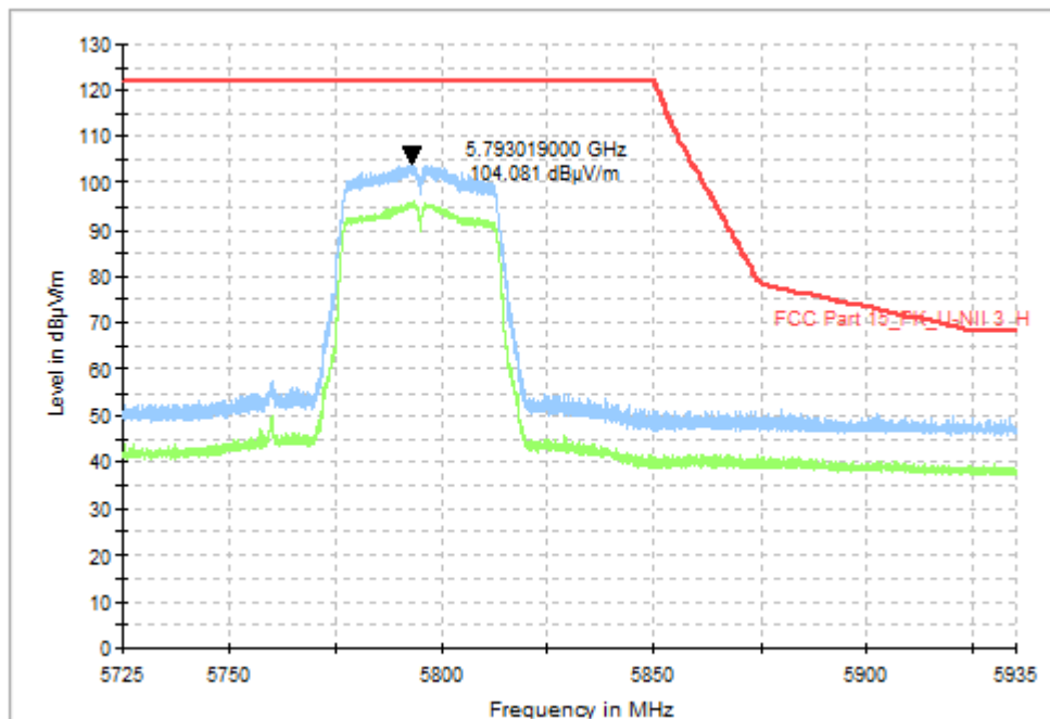
Fig. 64 Band Edges (802.11n-HT40, CH159 5795MHz)
