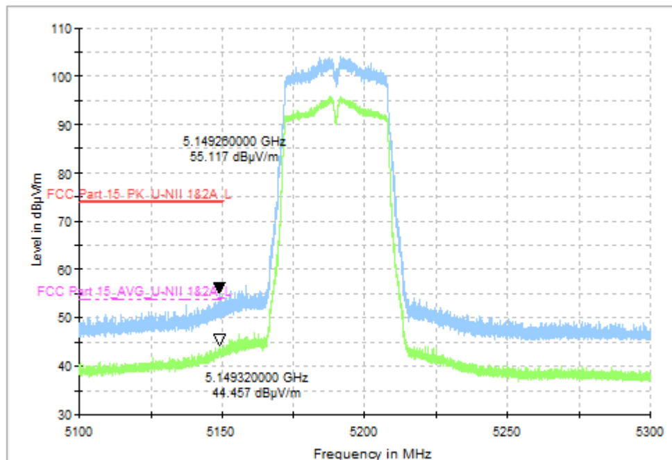
Fig. 59 Band Edges (802.11n-HT40, CH38 5190MHz)
