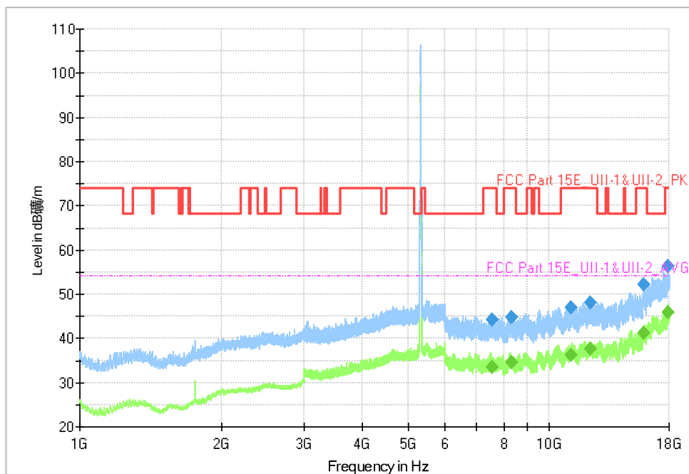
Fig. 76 Transmitter Spurious Emission (802.11a, CH64 5320MHz)
