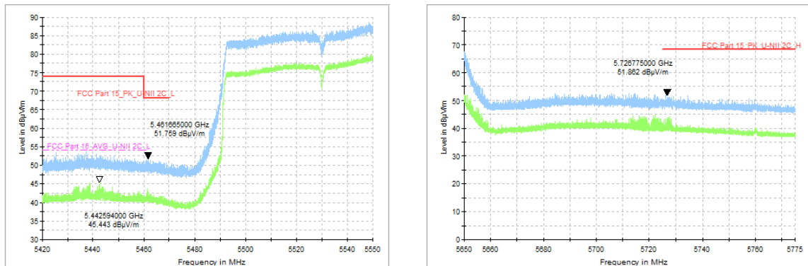
Fig. 70 Band Edges (802.11ac-VHT160, CH114 5570MHz)
