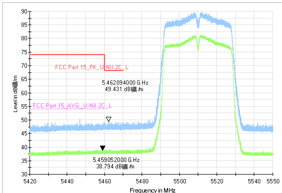
Fig. 61 Band Edges (802.11n-HT40, CH102 5510MHz)
