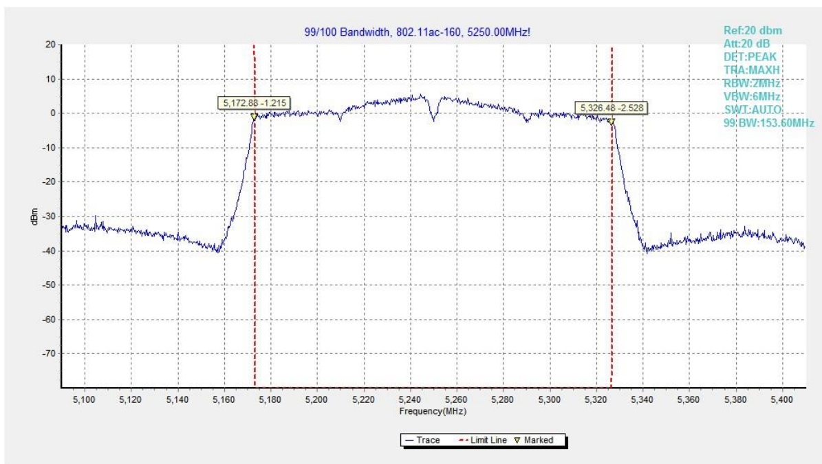
Fig. 51 99% Occupied Bandwidth (802. 11ac-VHT160, 5250MHz)
