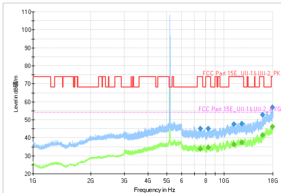
Fig. 72 Transmitter Spurious Emission (802.11a, CH40 5200MHz)
