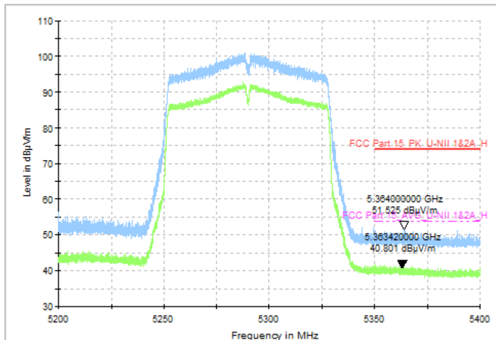
Fig. 66 Band Edges (802.11ac-VHT80, CH58 5290MHz)
