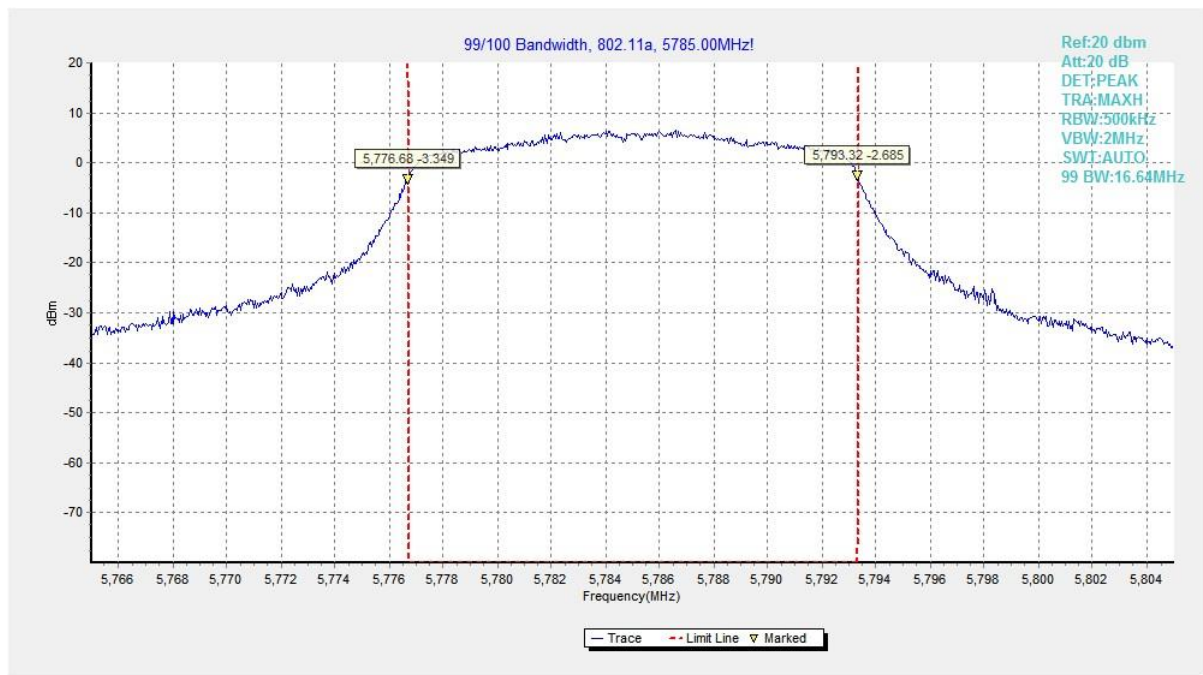
Fig. 37 99% Occupied Bandwidth (802.11a, 5785MHz)
