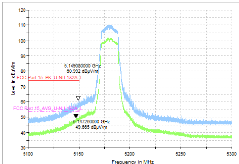
Fig. 53 Band Edges (802.11a, CH36 5180MHz)
