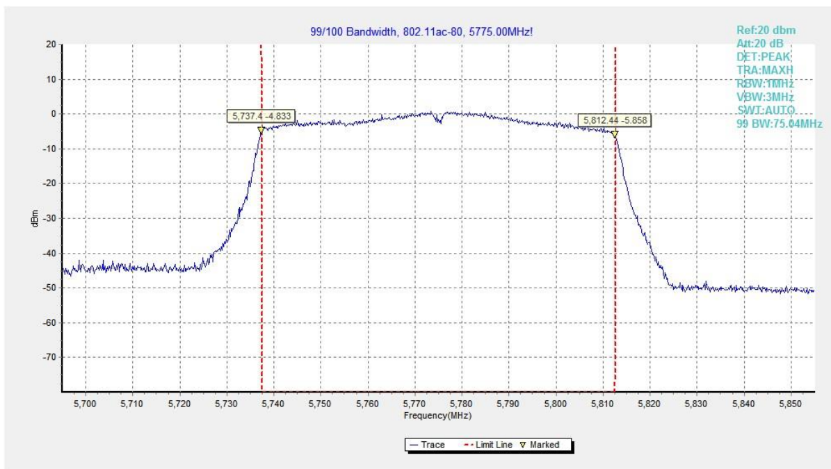
Fig. 50 99% Occupied Bandwidth (802. 11ac-VHT80, 5775MHz)
