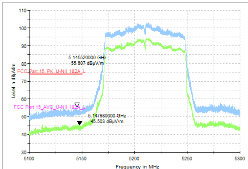
Fig. 65 Band Edges (802.11ac-VHT80, CH42 5210MHz)
