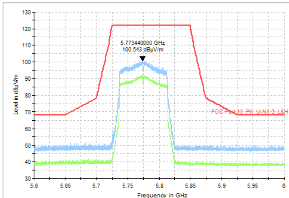
Fig. 68 Band Edges (802.11ac-VHT80, CH155 5775MHz)
