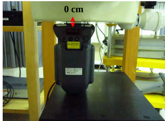
Fig.3 EUT front to flat phantom
