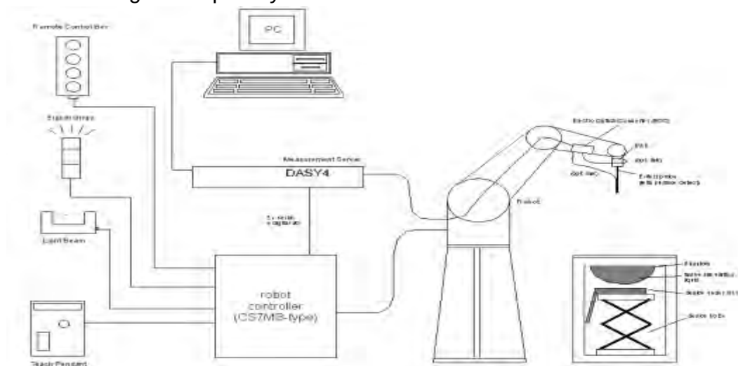
Fig.a The block diagram of SAR system
