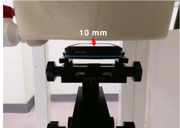
Fig.12 EUT Front side to flat phantom
