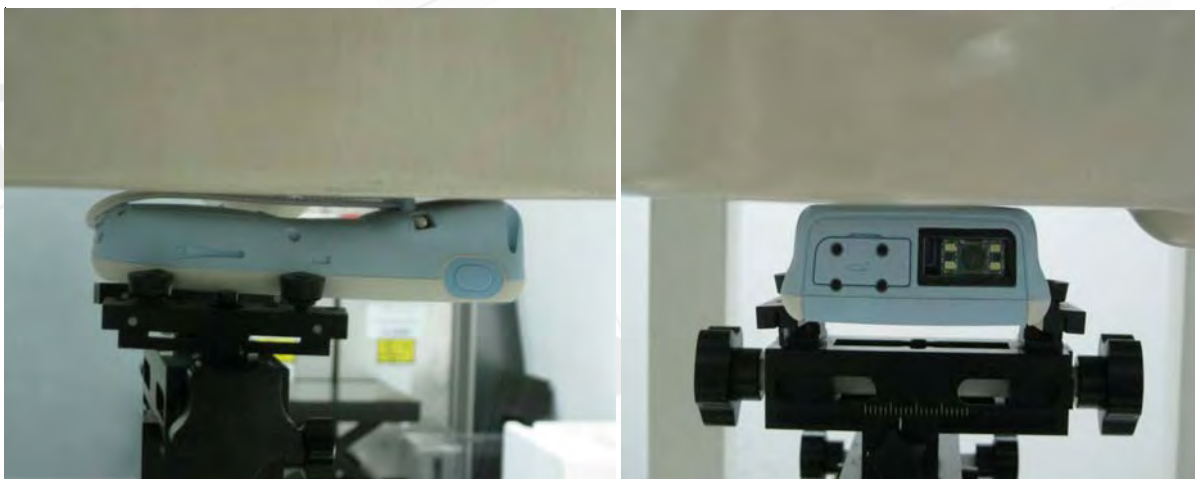
Fig.4 Back side of EUT is paralleled with flat phantom, separating 0cm between the back of the EUT and the flat phantom.
