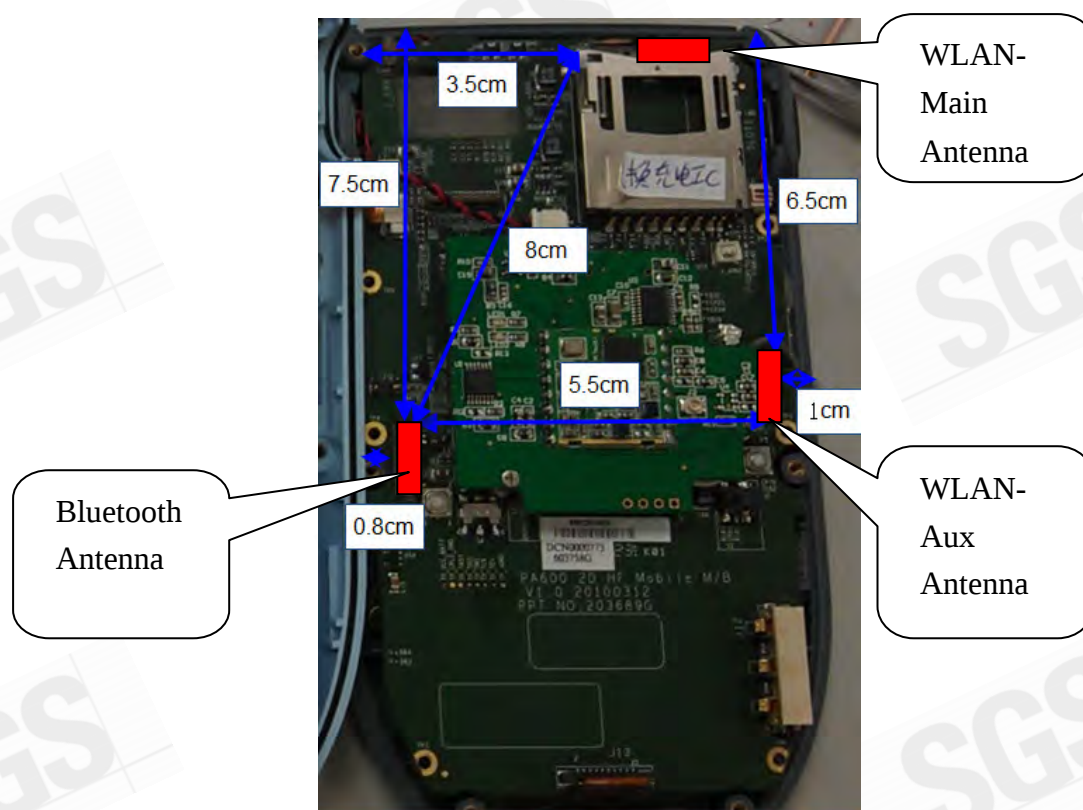
Fig.9 Antenna position & distance
