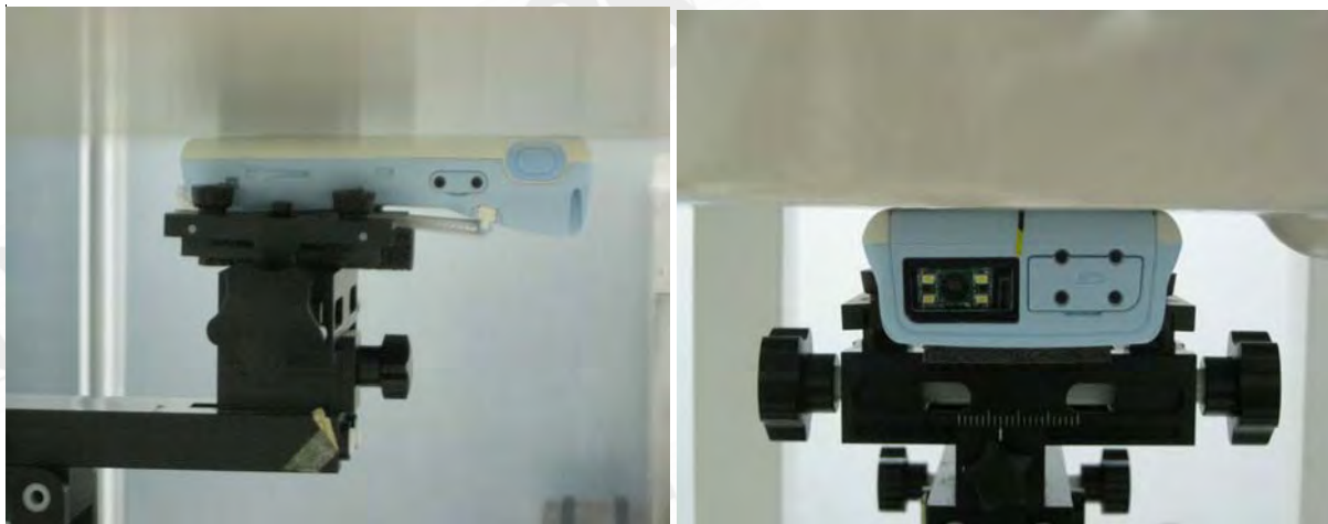
Fig.3 Front side of EUT is paralleled with flat phantom, separating 0cm between the back of the EUT and the flat phantom.
