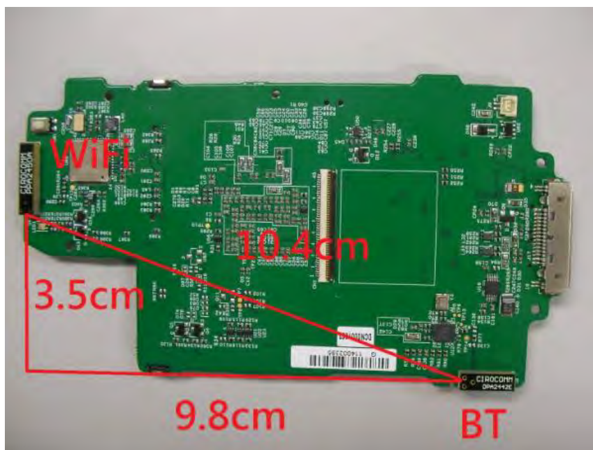
Fig.8 Antenna position of EUT
