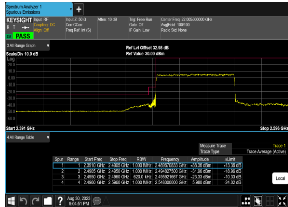
N41(60M)_DFT-s-OFDM_BPSK_Outer_Full_Low_CH
