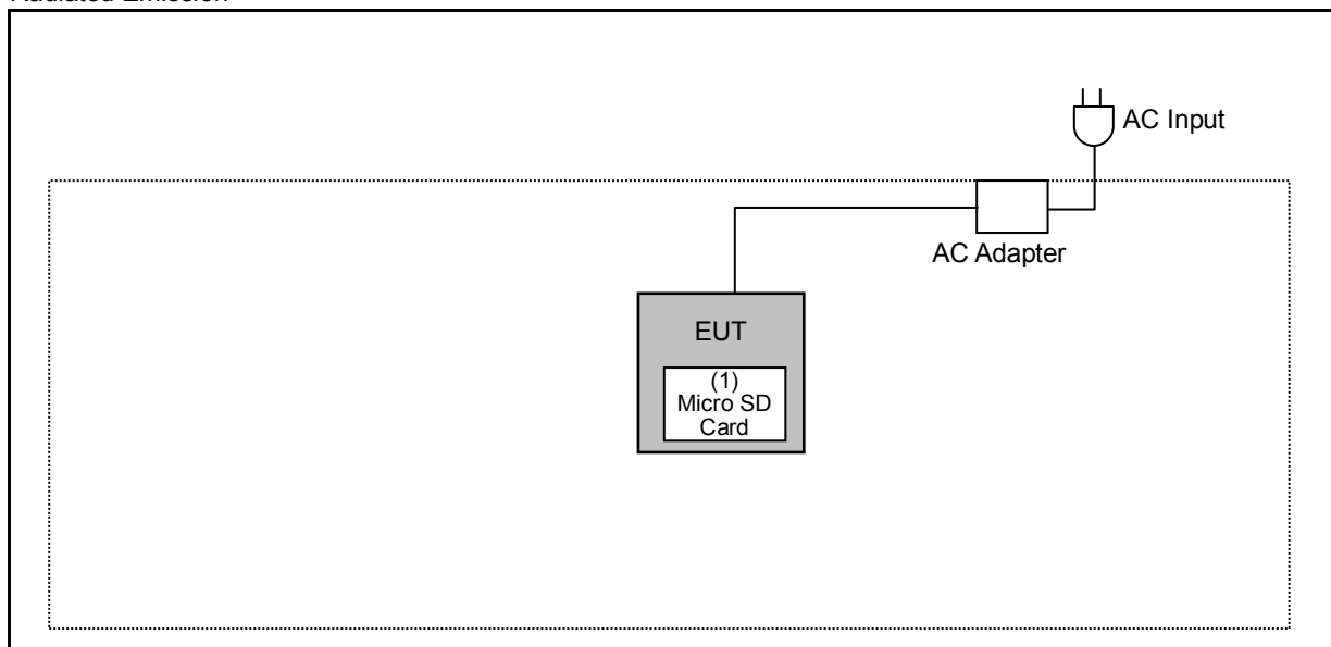
Radiated Emission
