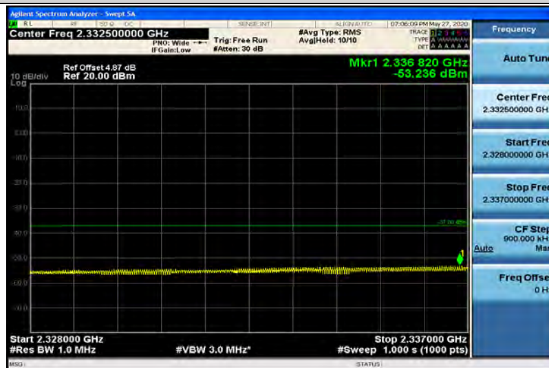
Band40-5MHz-QPSK-39200-1RB#24-Range8:2328~2337MHz
