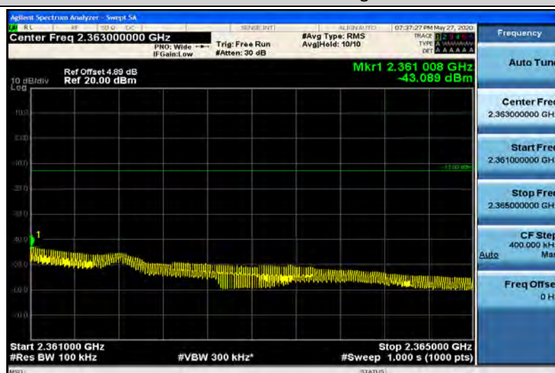
Band40-5MHz-QPSK-39225-1RB#0-Range13:2361~2365MHz
