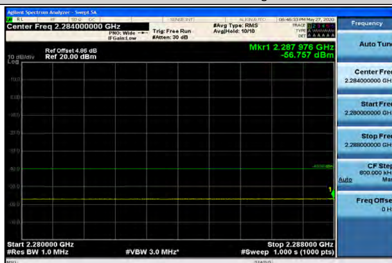
Band40-5MHz-16QAM-39175-1RB#24-Range1:2280~2288MHz
