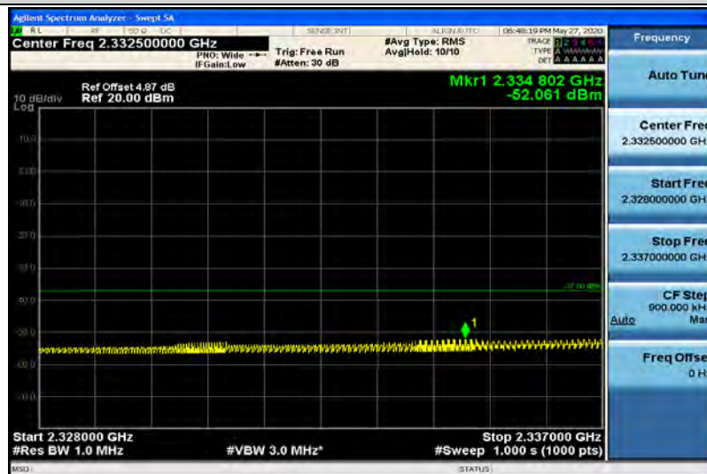
Band40-5MHz-16QAM-39175-1RB#24-Range8:2328~2337MHz
