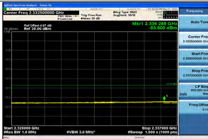
Band40-5MHz-QPSK-39225-1RB#24-Range8:2328~2337MHz
