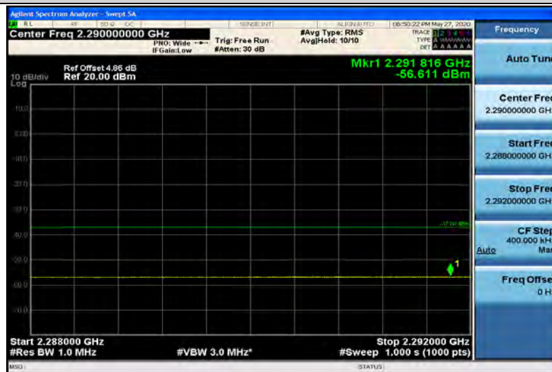
Band40-5MHz-QPSK-39175-1RB#0-Range2:2288~2292MHz
