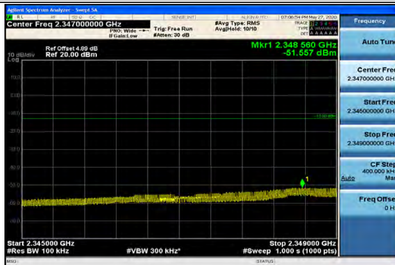
Band40-5MHz-QPSK-39200-1RB#24-Range11:2345~2349MHz
