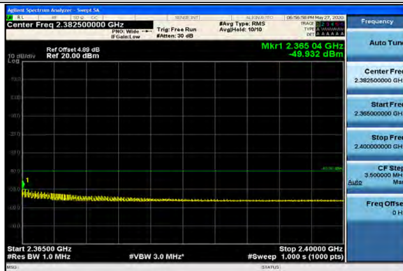
Band40-5MHz-16QAM-39175-1RB#0-Range14:2365~2400MHz
