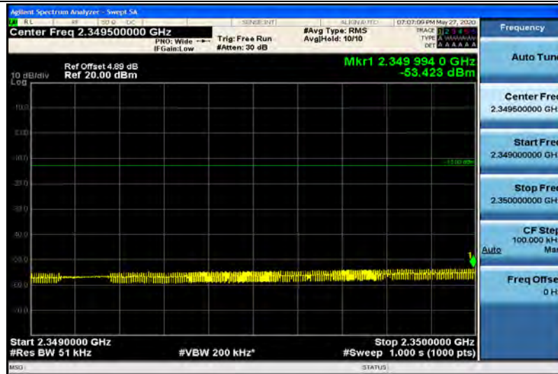
Band40-5MHz-QPSK-39200-1RB#24-Range12:2349~2350MHz
