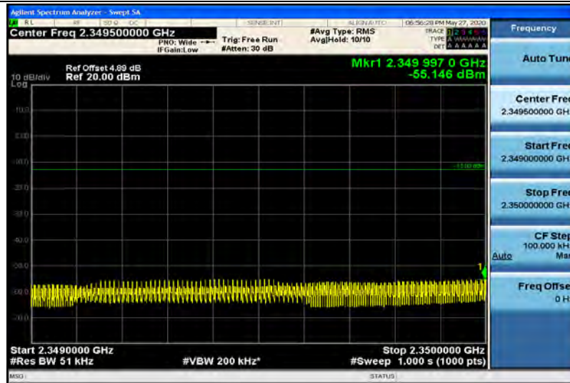
Band40-5MHz-16QAM-39175-1RB#0-Range12:2349~2350MHz
