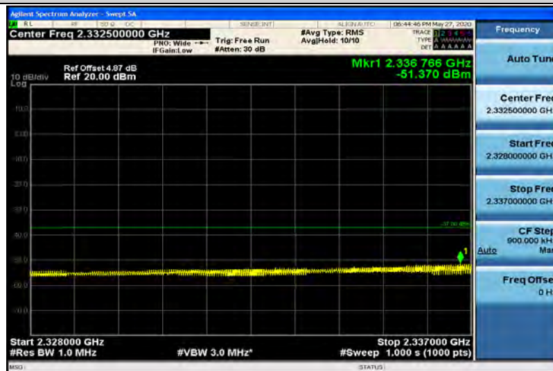
Band40-5MHz-QPSK-39175-1RB#24-Range8:2328~2337MHz
