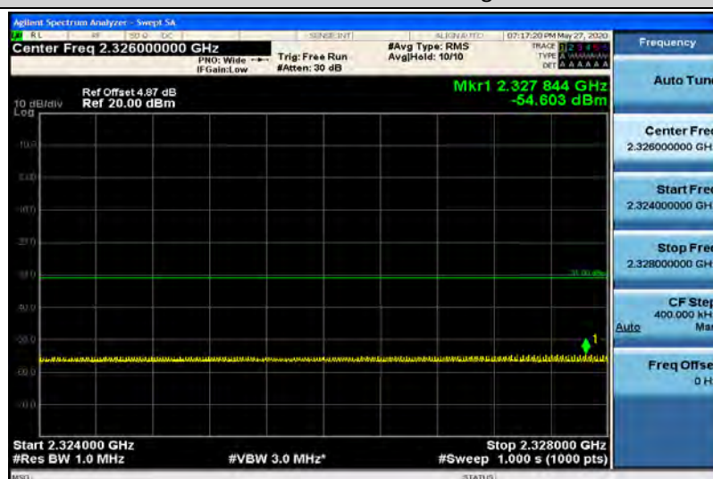
Band40-5MHz-16QAM-39200-1RB#0-Range7:2324~2328MHz
