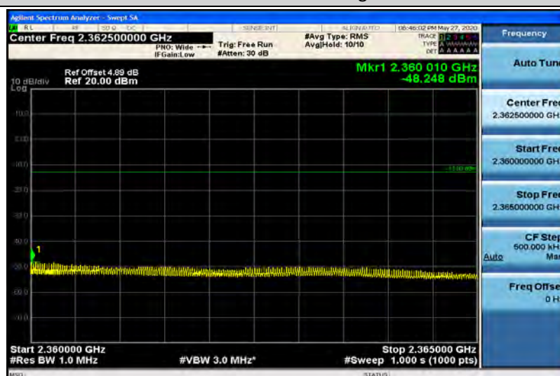
Band40-5MHz-QPSK-39175-1RB#24-Range13:2360~2365MHz
