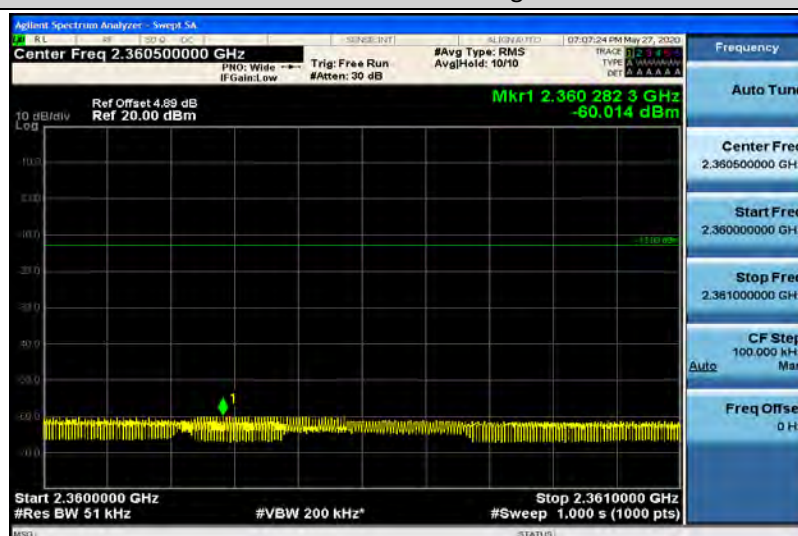
Band40-5MHz-QPSK-39200-1RB#24-Range13:2360~2361MHz
