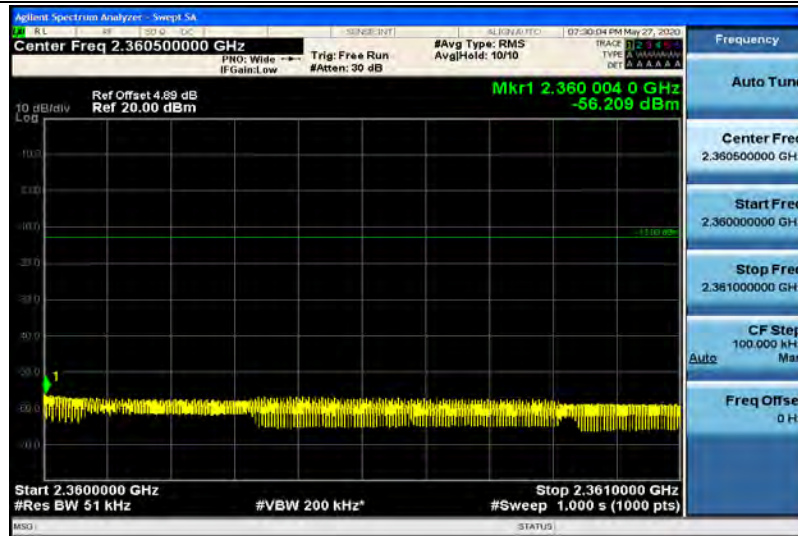
Band40-5MHz-QPSK-39225-1RB#24-Range12:2360~2361MHz
