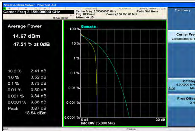
Band40-10MHz-16QAM-39200-1RB#0
