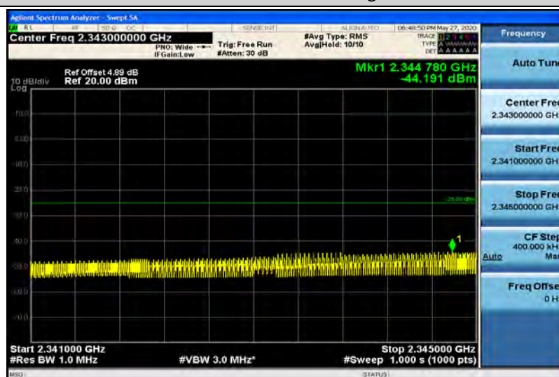
Band40-5MHz-16QAM-39175-1RB#24-Range10:2341~2345MHz
