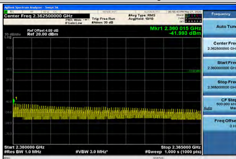
Band40-5MHz-16QAM-39175-1RB#0-Range13:2360~2365MHz
