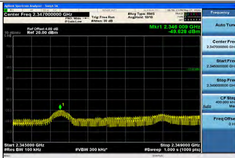
Band40-5MHz-16QAM-39175-1RB#0-Range11:2345~2349MHz
