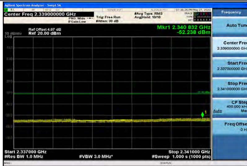
Band40-5MHz-QPSK-39225-1RB#0-Range9:2337~2341MHz
