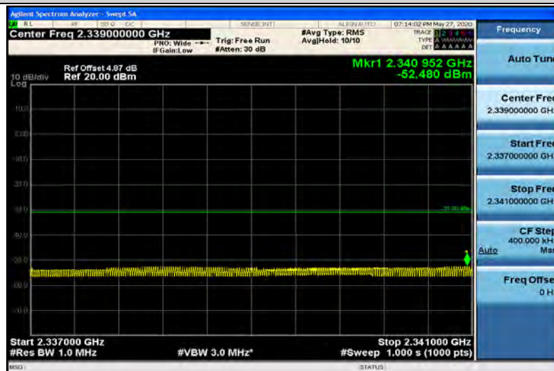
Band40-5MHz-QPSK-39200-1RB#0-Range10:2341~2345MHz
