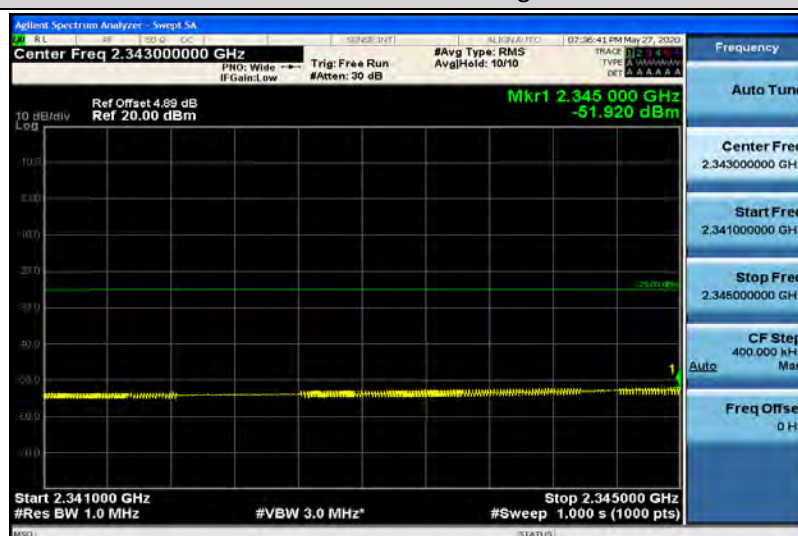
Band40-5MHz-QPSK-39225-1RB#0-Range10:2341~2345MHz
