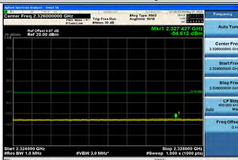
Band40-5MHz-QPSK-39200-1RB#24-Range7:2324~2328MHz
