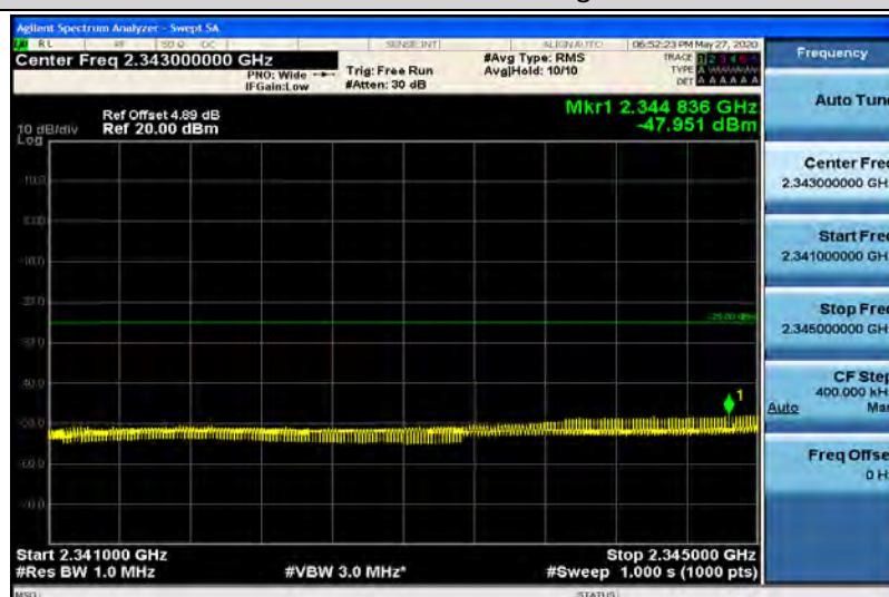
Band40-5MHz-QPSK-39175-1RB#0-Range10:2341~2345MHz
