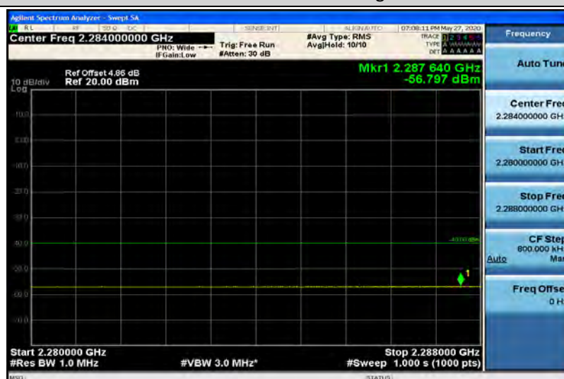
Band40-5MHz-16QAM-39200-1RB#24-Range1:2280~2288MHz
