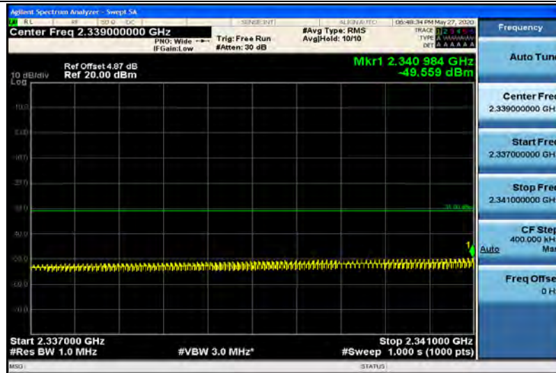
Band40-5MHz-16QAM-39175-1RB#24-Range9:2337~2341MHz
