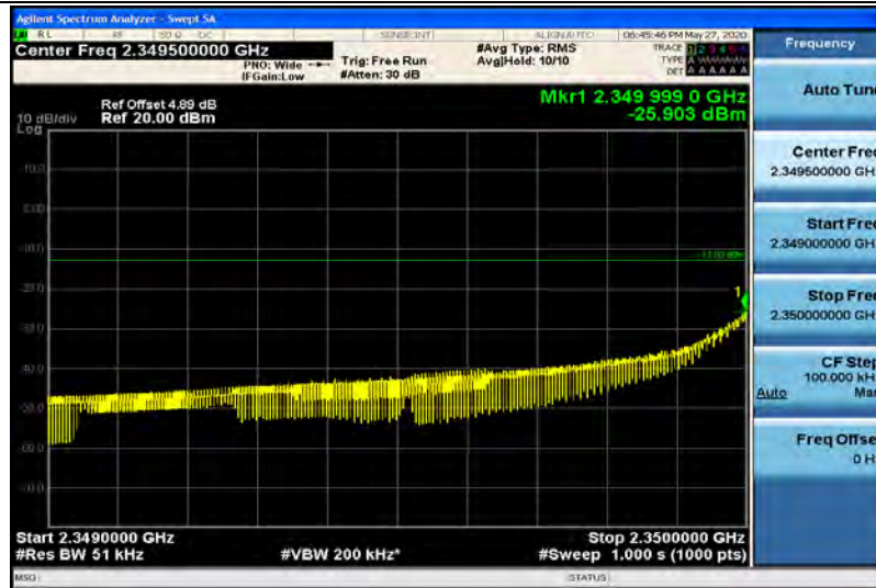
Band40-5MHz-QPSK-39175-1RB#24-Range12:2349~2350MHz
