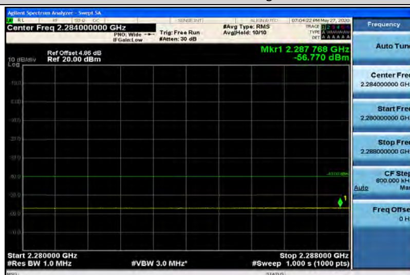
Band40-5MHz-QPSK-39200-1RB#24-Range1:2280~2288MHz
