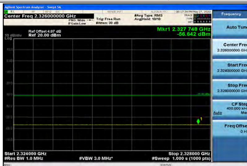
Band40-10MHz-16QAM-39200-1RB#49-Range7:2324~2328MHz
