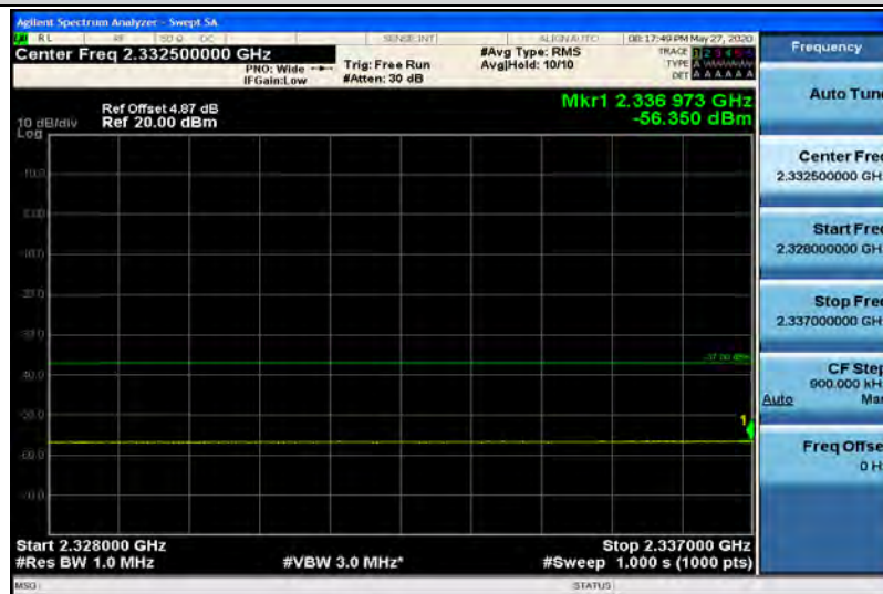
Band40-10MHz-16QAM-39200-1RB#49-Range8:2328~2337MHz
