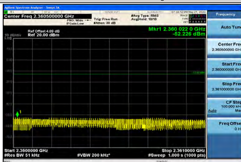
Band40-5MHz-16QAM-39200-1RB#0-Range13:2360~2361MHz
