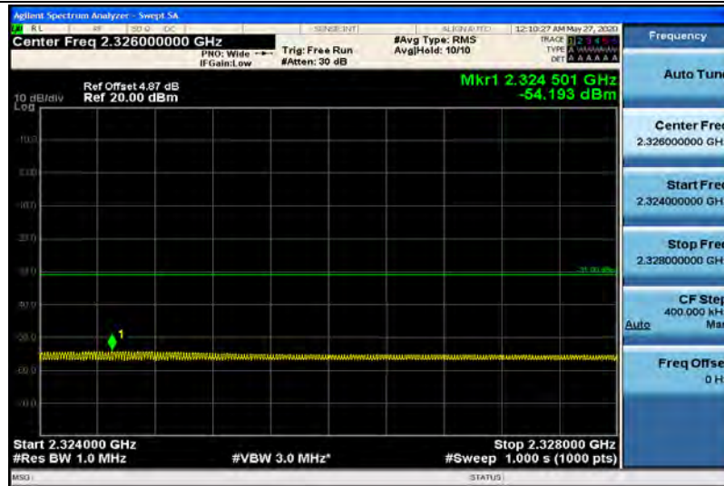
Band40-5MHz-QPSK-38725-1RB#24-Range9:2324~2328MHz
