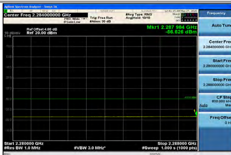
Band40-5MHz-16QAM-38750-1RB#0-Range1:2280~2288MHz
