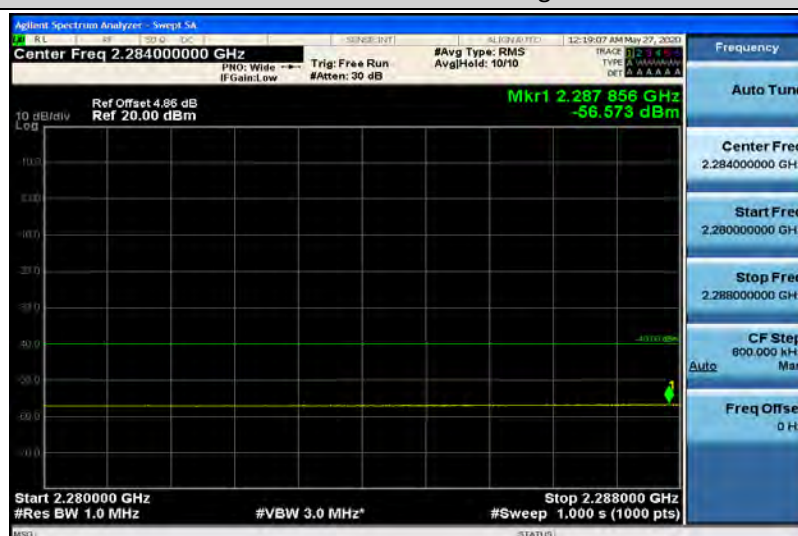
Band40-5MHz-16QAM-38725-1RB#0-Range1:2280~2288MHz
