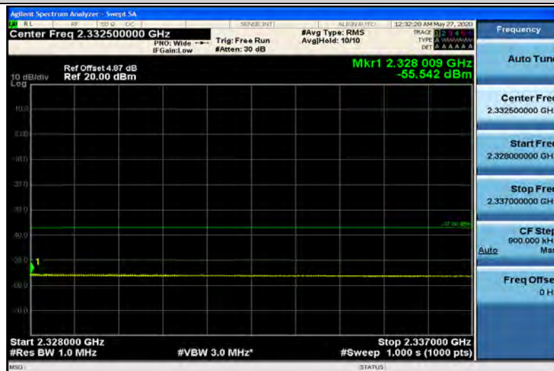
Band40-5MHz-QPSK-38750-1RB#24-Range11:2328~2337MHz
