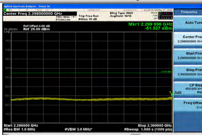
Band40-5MHz-16QAM-38725-1RB#0-Range4:2296~2300MHz
