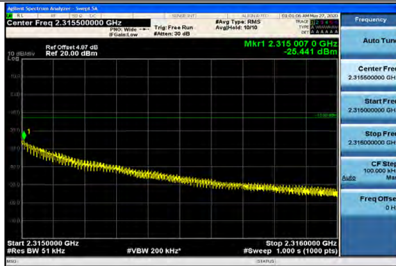
Band40-5MHz-QPSK-38775-1RB#0-Range6:2315~2316MHz
