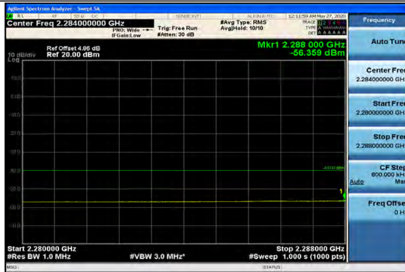
Band40-5MHz-16QAM-38725-1RB#24-Range2:2288~2292MHz
