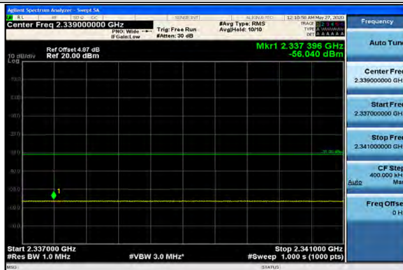
Band40-5MHz-QPSK-38725-1RB#24-Range11:2337~2341MHz
