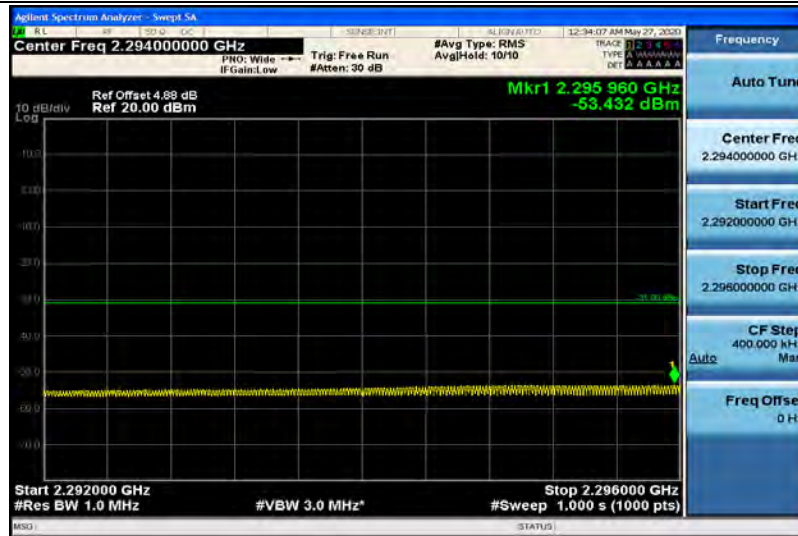
Band40-5MHz-16QAM-38750-1RB#24-Range3:2292~2296MHz
