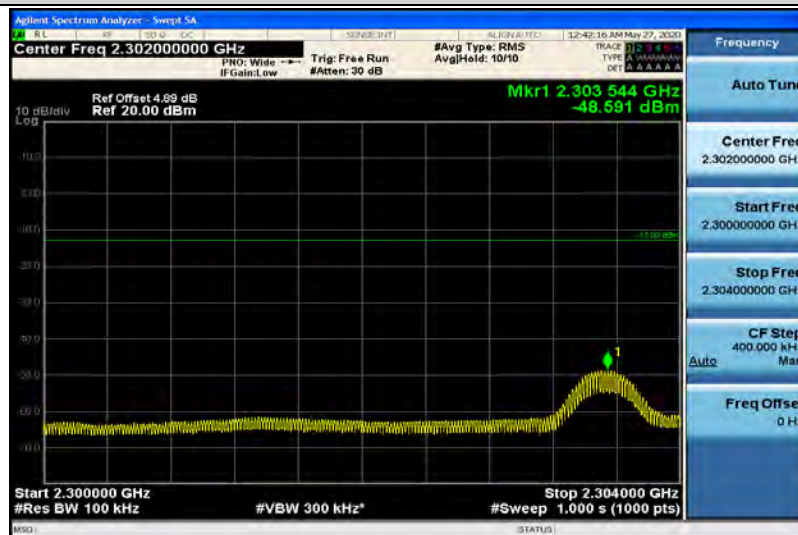
Band40-5MHz-16QAM-38750-1RB#0-Range5:2300~2304MHz
