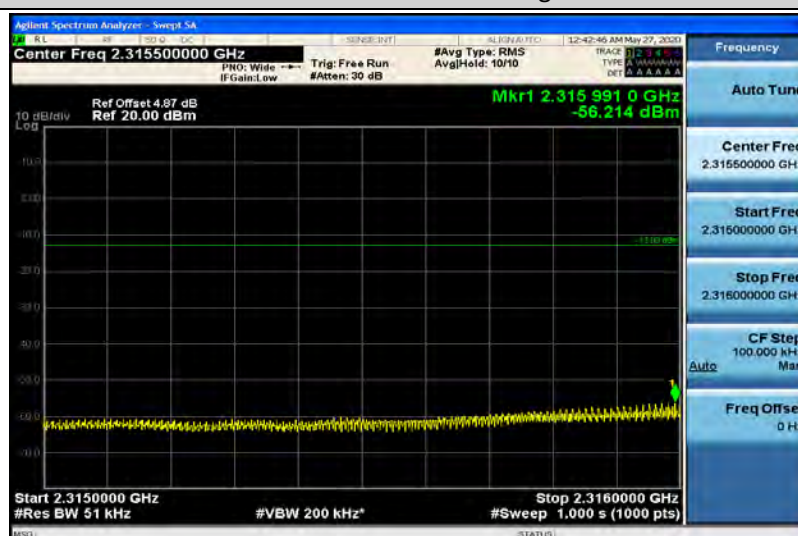
Band40-5MHz-16QAM-38750-1RB#0-Range7:2315~2316MHz
