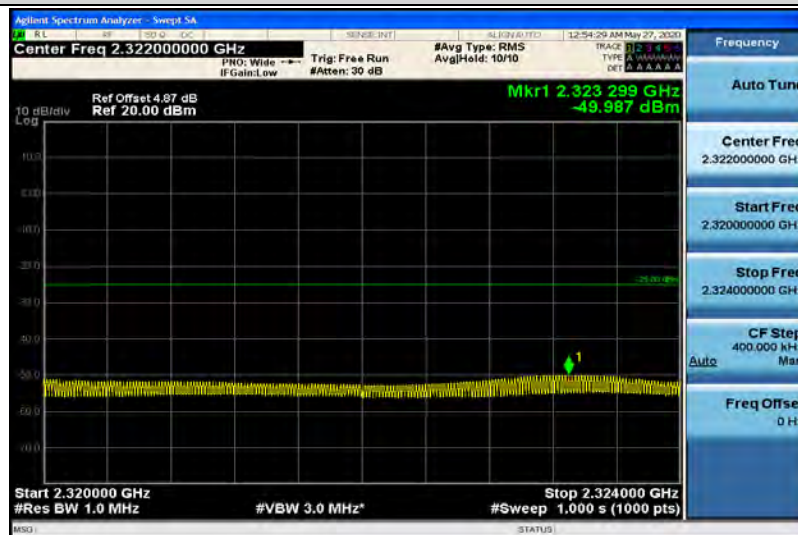
Band40-5MHz-QPSK-38775-1RB#24-Range8:2320~2324MHz
