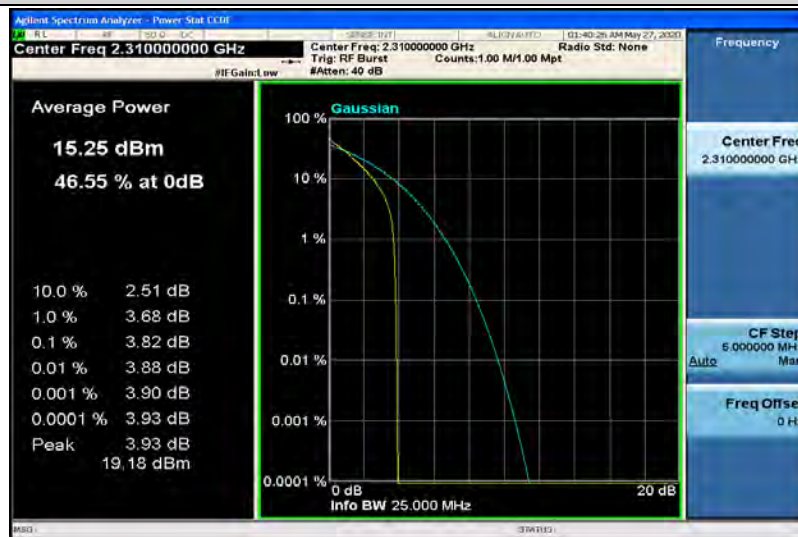
Band40-10MHz-16QAM-38750-1RB#0
