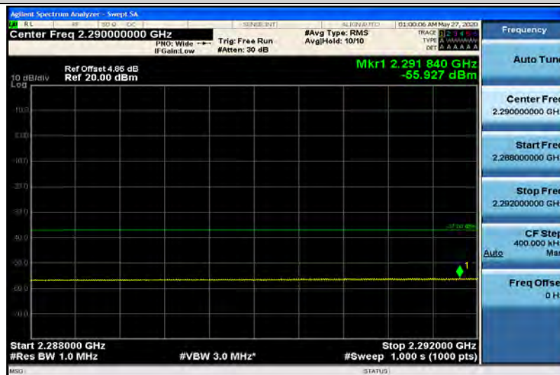
Band40-5MHz-QPSK-38775-1RB#0-Range2:2288~2292MHz
