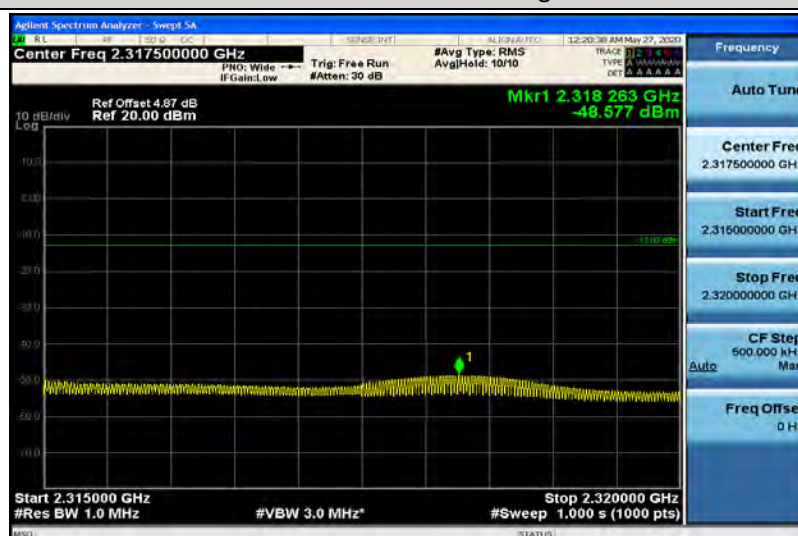
Band40-5MHz-16QAM-38725-1RB#0-Range7:2315~2320MHz
