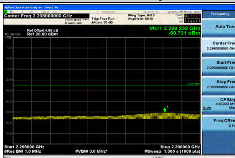
Band40-5MHz-16QAM-38750-1RB#0-Range4:2296~2300MHz
