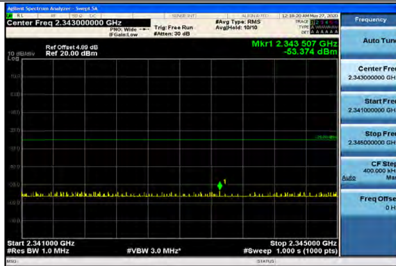
Band40-5MHz-QPSK-38725-1RB#0-Range12:2341~2345MHz
