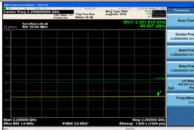
Band40-5MHz-QPSK-38750-1RB#0-Range2:2288~2292MHz
