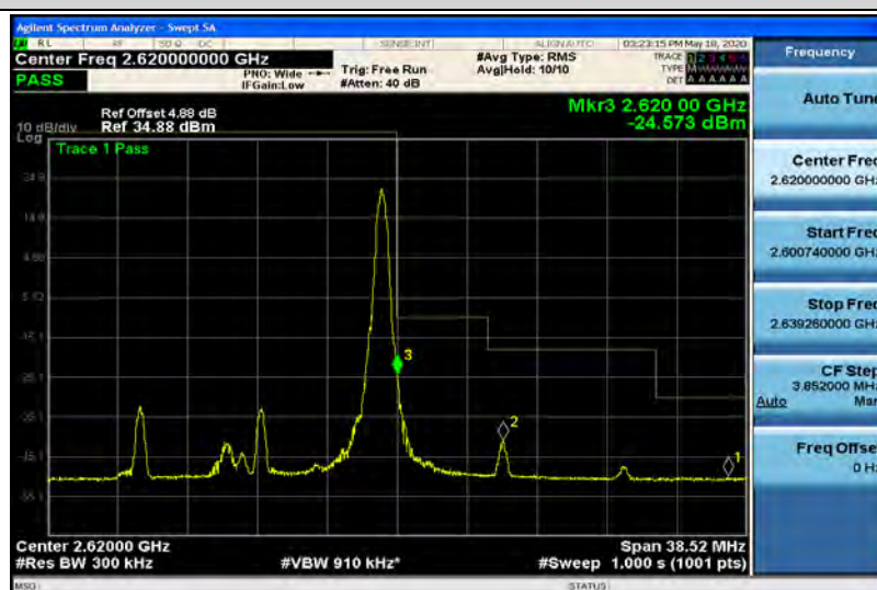
Band38-15MHz-16QAM-38175-75RB#0
