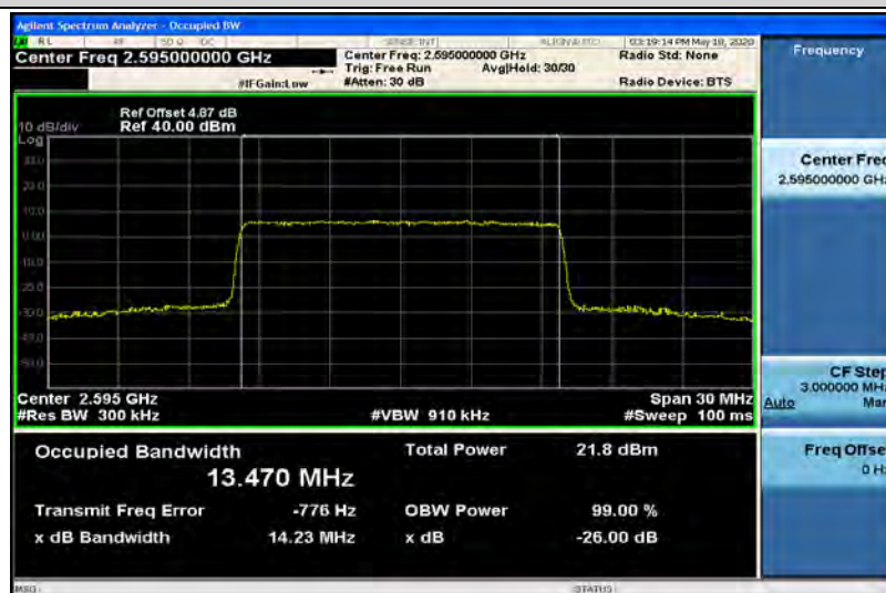
Band38-15MHz-16QAM-38175-75RB#0-13.466
