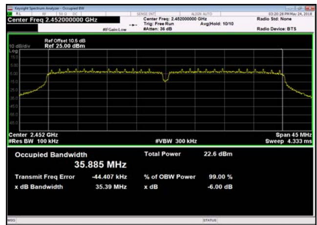
802.11n(HT40),2452MHz,
