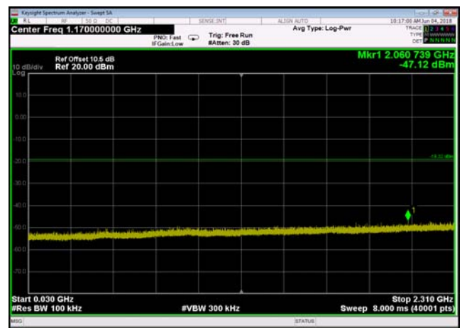
,Plot 3,30MHz~2310MHz-802.11g,2462MHz
