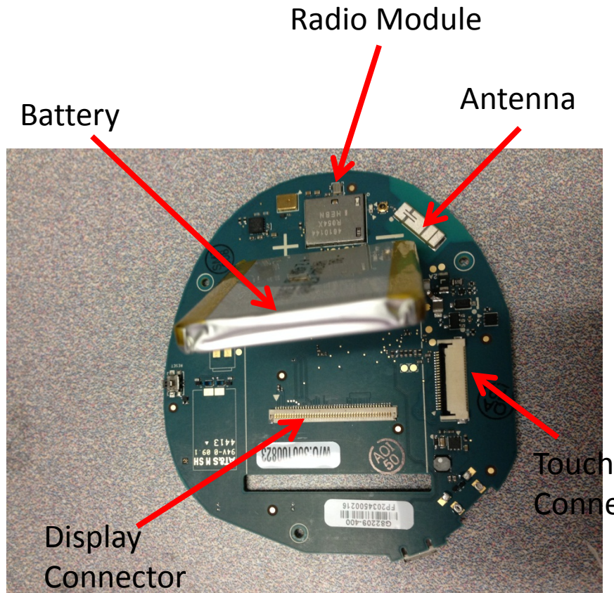
Inside PCB TOP View
