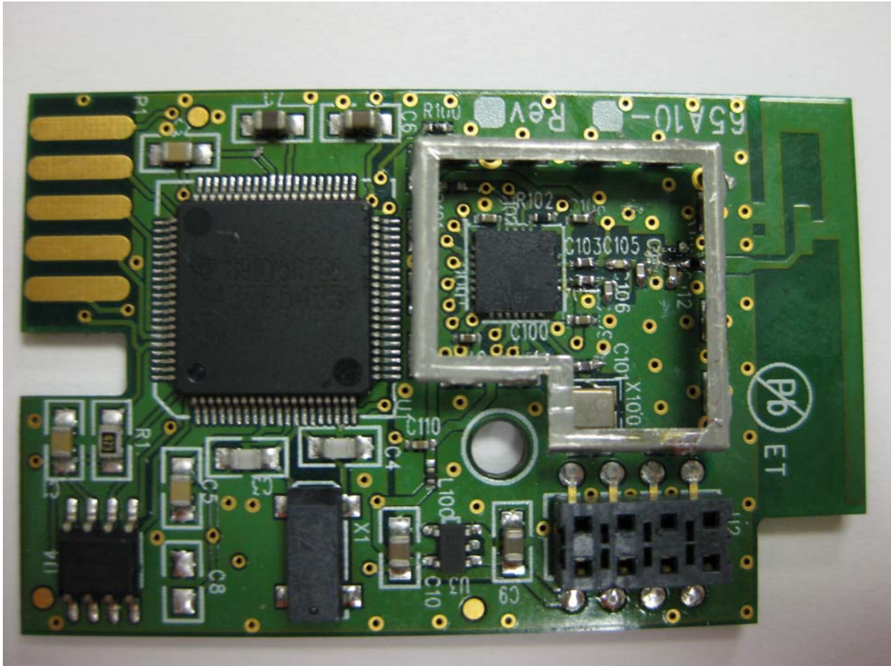
Internal View #2 – Shield Removed
