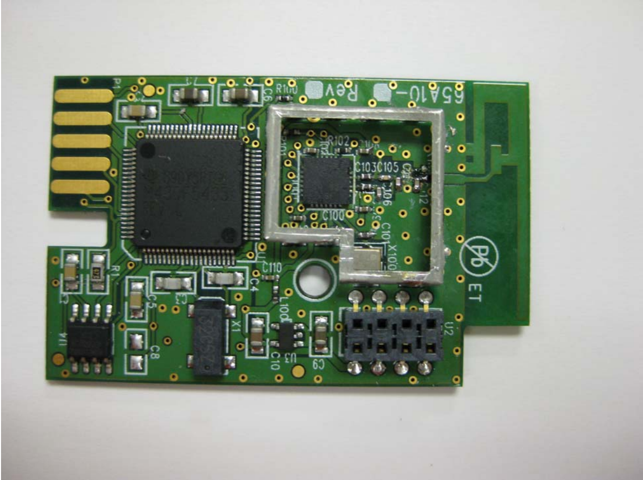
Internal View #1 – Shield Removed
