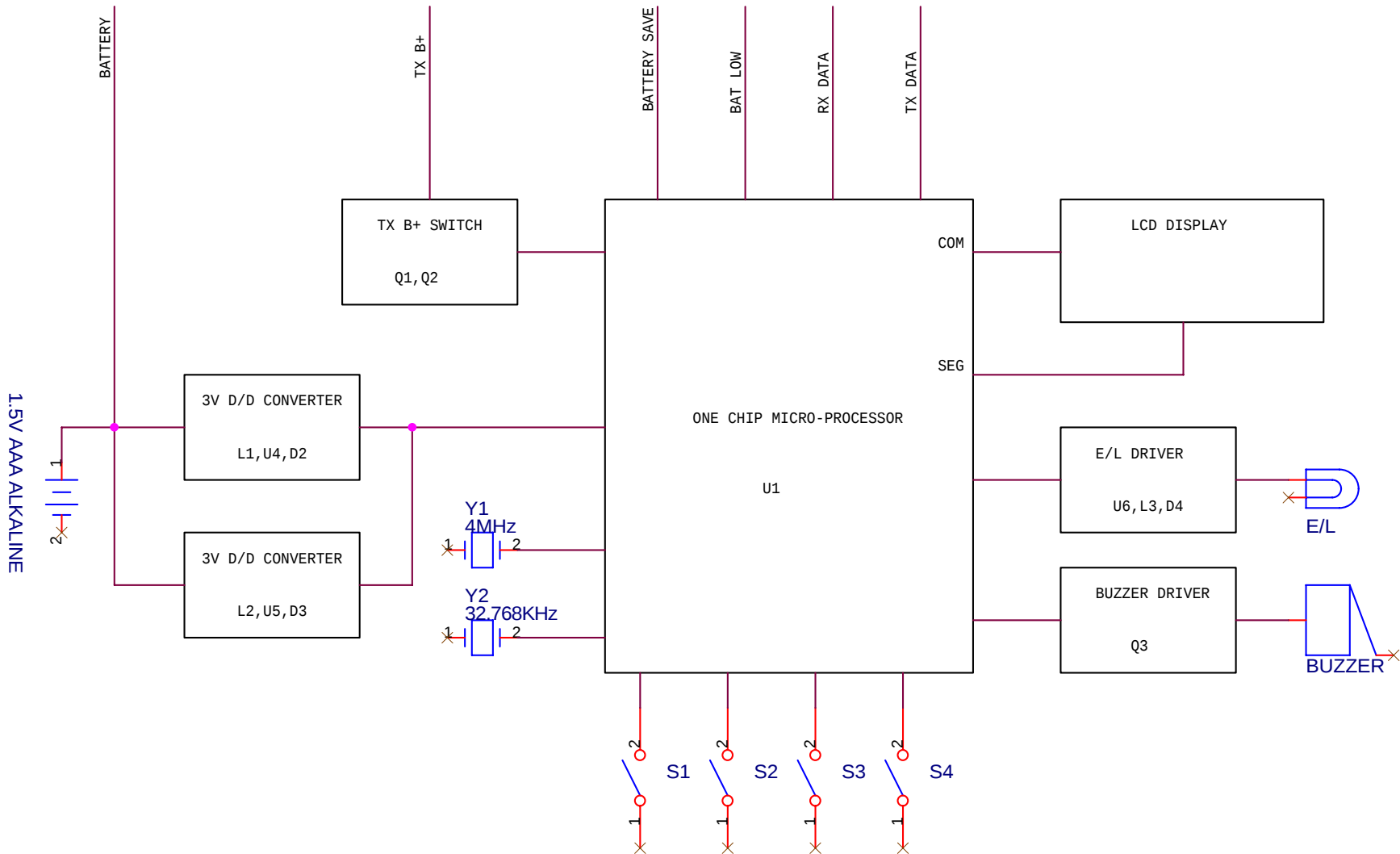
BLOCK DIAGRAM OF TW-03R REMOTE UNIT(CONTROL BOARD)
