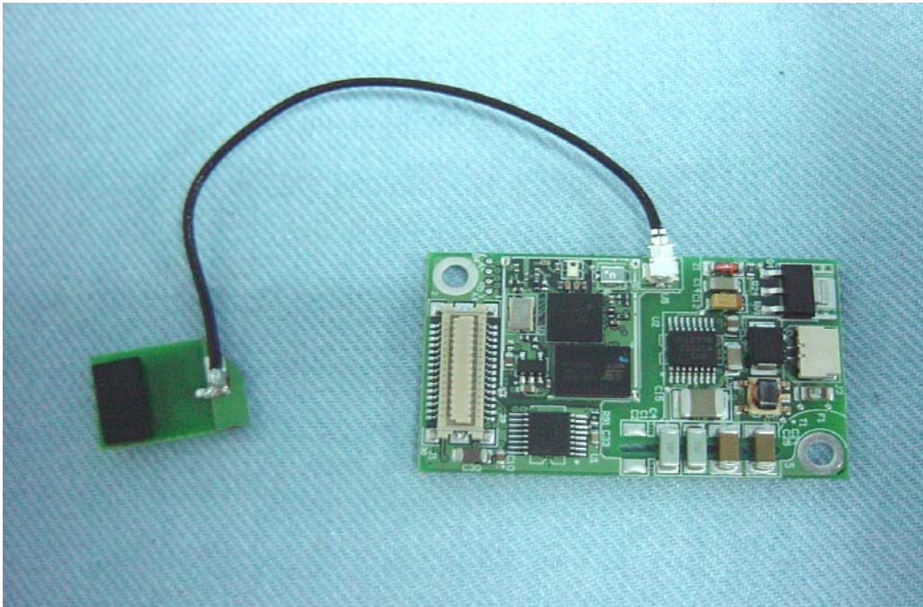
Front of Bluetooth Module with Antenna
