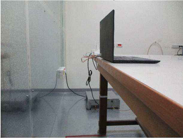
Conduction_Setup
