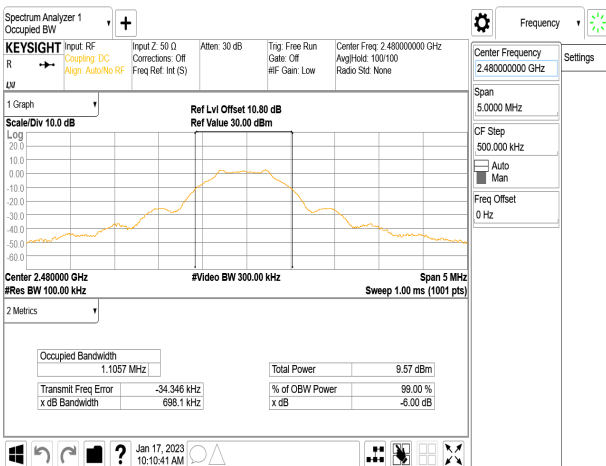
OBW_BLE 1M_HighCH39-2480MHz
