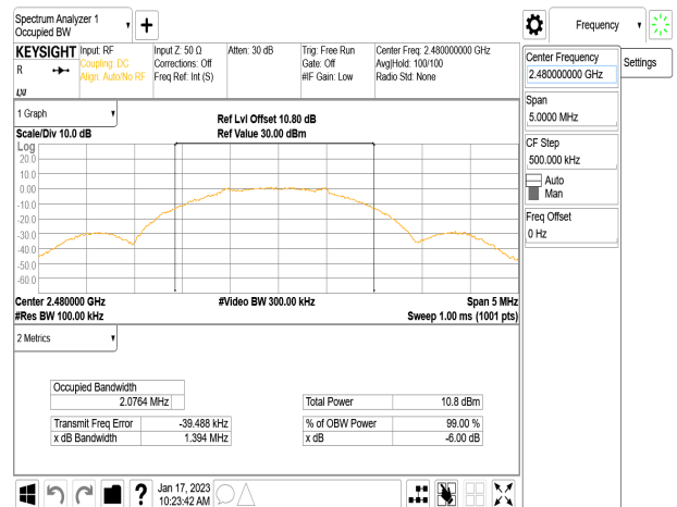
OBW_BLE 2M_HighCH39-2480MHz
